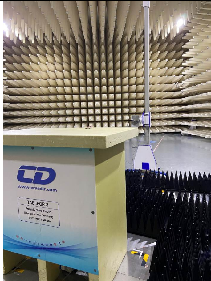
Radiated Emissions Test Setup (above1GHz)
