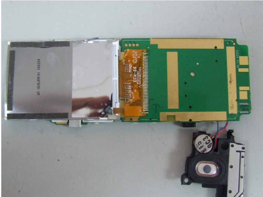
PCB Back View
