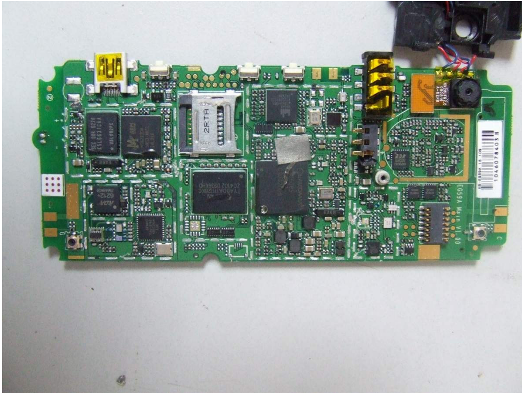
PCB without Shield Front View
