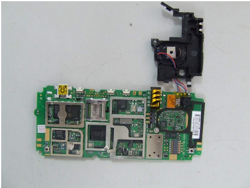
PCB with Shield Front View
