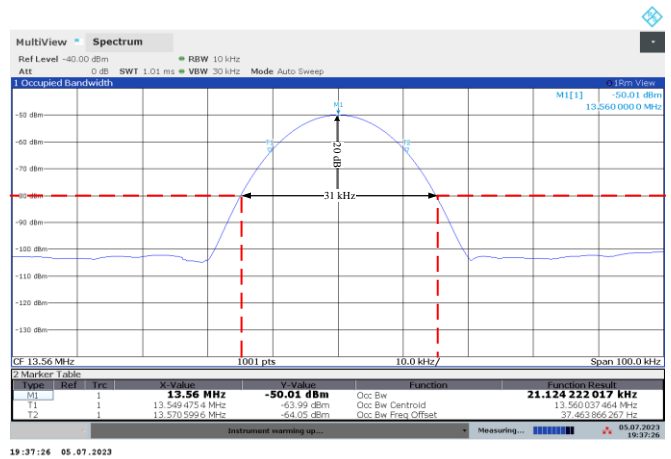
Figure 7.4-2: 20 dB bandwidth
