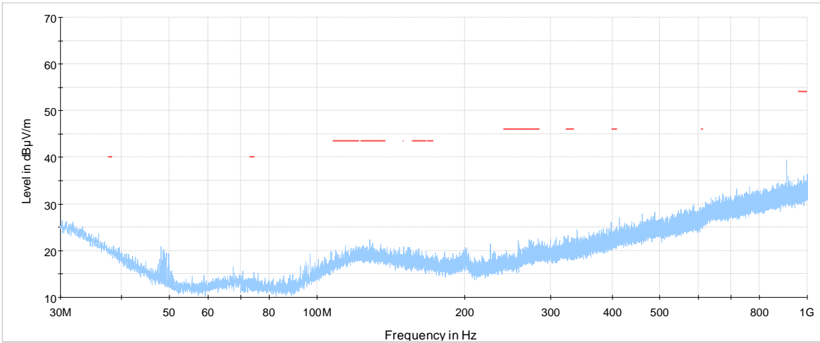
RE 30 MHz to 1 GHz MT6 MTRFID Round RFID ON — Preview Result 1-PK+ — FCC 15.209 and RSS-210 limit line RstrB ◆ Final_Result QPK
