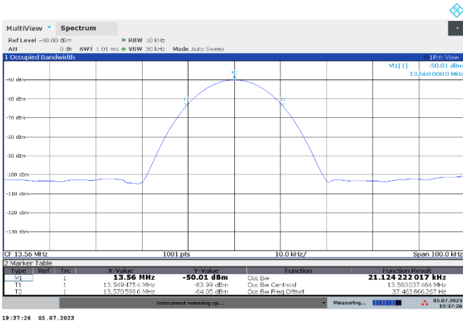
Figure 7.4-1: 99% bandwidth
