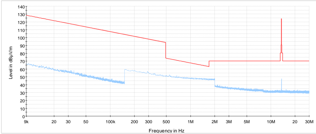
RE 9K to 30 MHz MT6 MTRFID Round E feild — Preview Result 1-PK+ • Critical_Freqs PK+ — 13.56 MHz mask FCC15.225 at3m-E field ◆ Final_Result QPK
