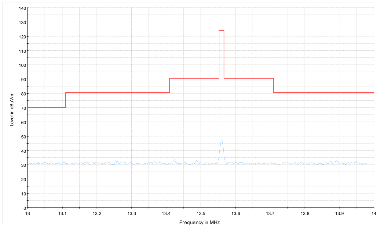
SPR 13 MHz to 14 MHz MT6 MTRFID Round E feild — Preview Result 1-PK+ — 13.56 MHz mask FCC15.225 at3m-E field
