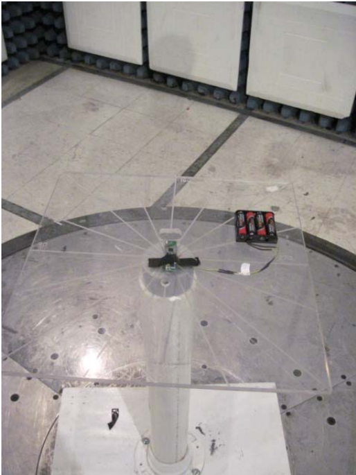
Close-up of Radiated Emissions Setup
