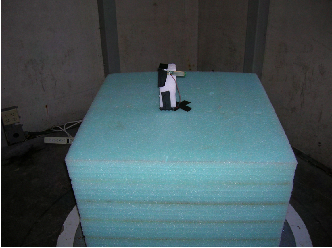
Radiated Measurements
