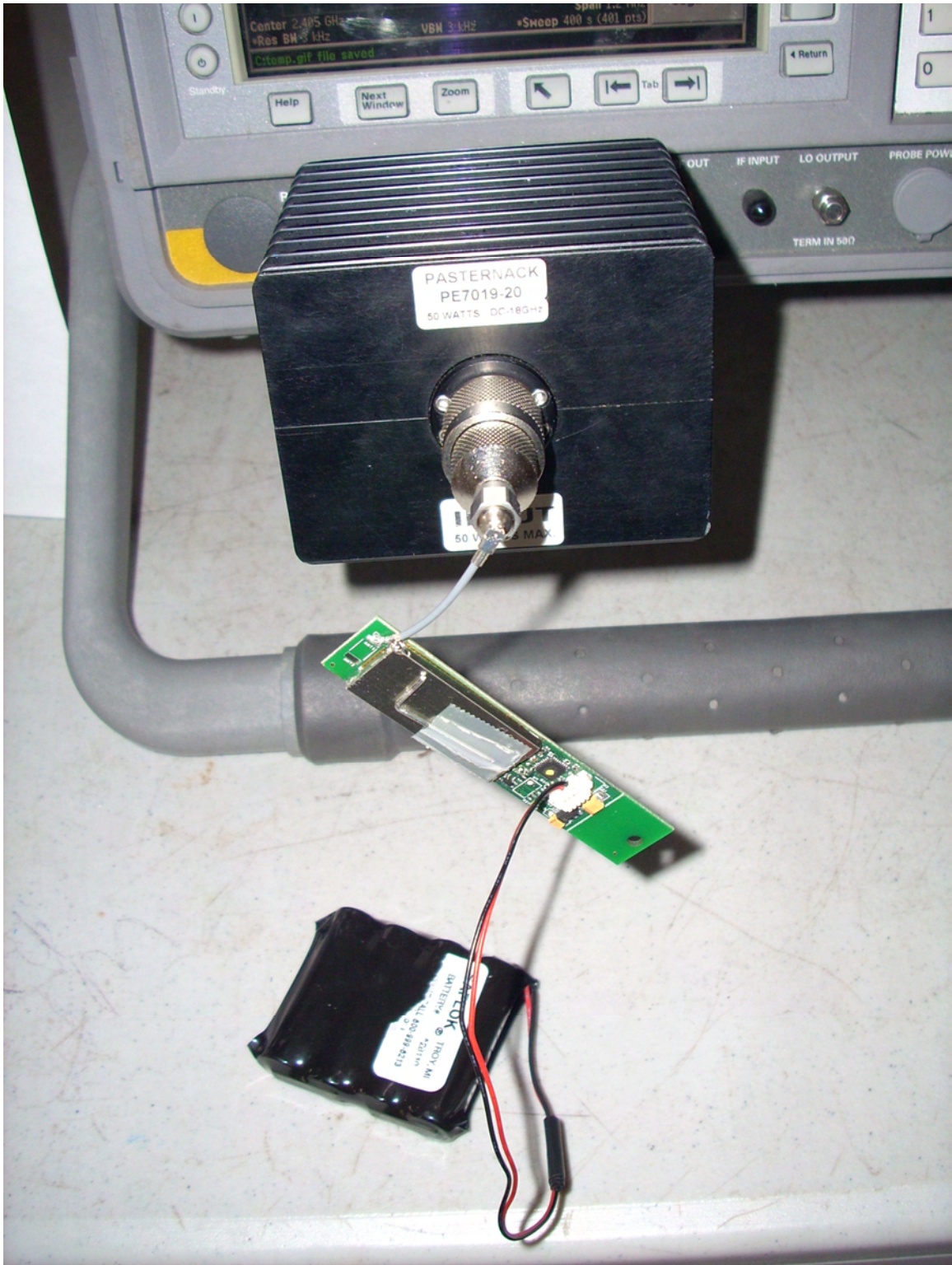
Conducted Measurements
