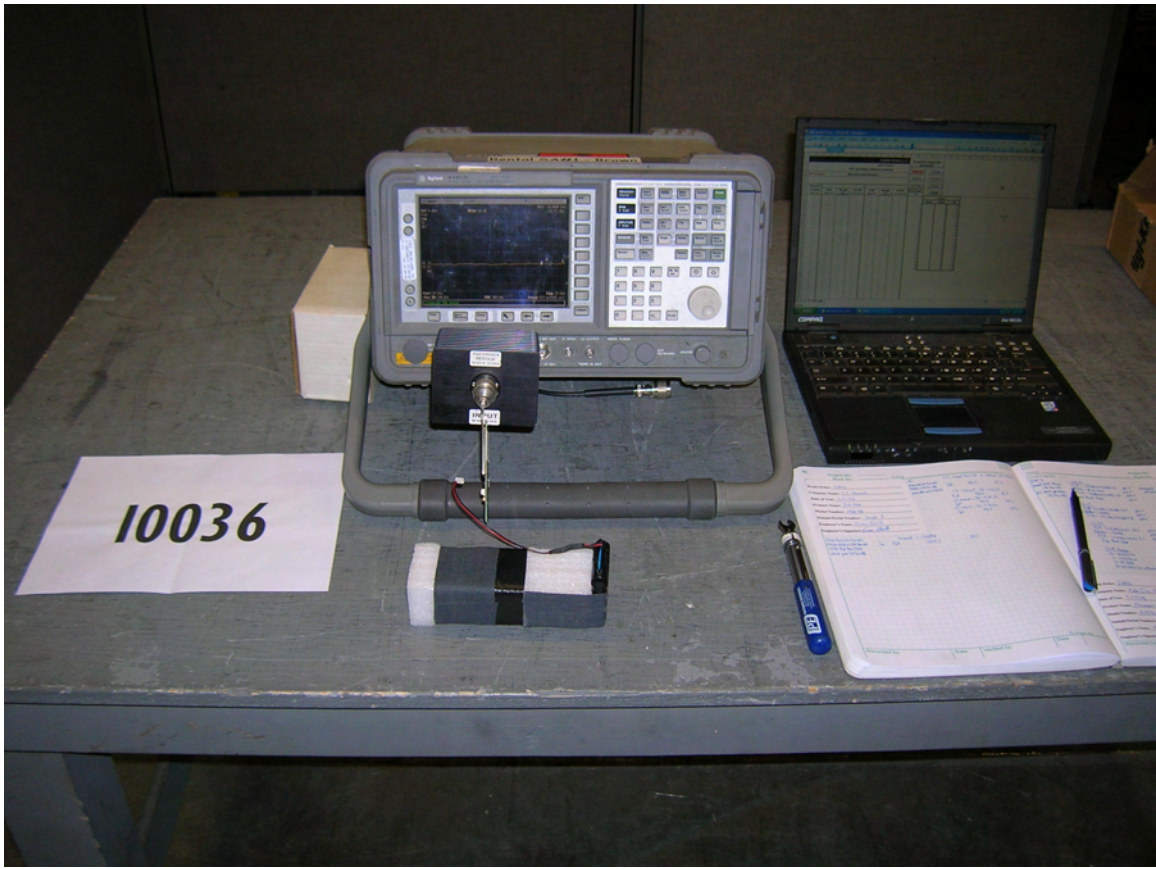
Conducted Measurements
