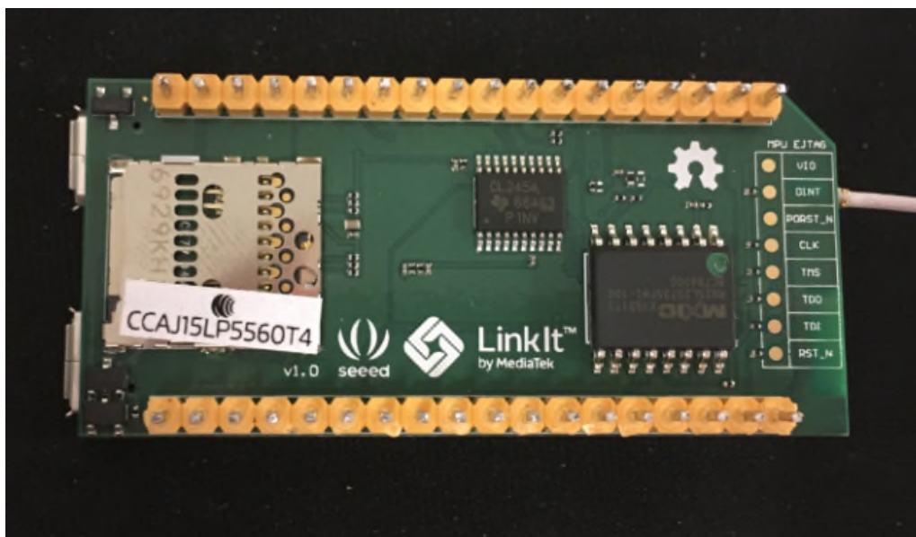
Figure 6: Module with Shields - Back
