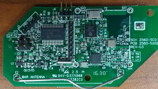
RF PWB Component side
