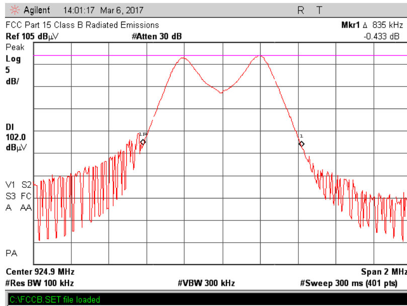
Figure 2.3.9-3 - High Channel Bandwidth
