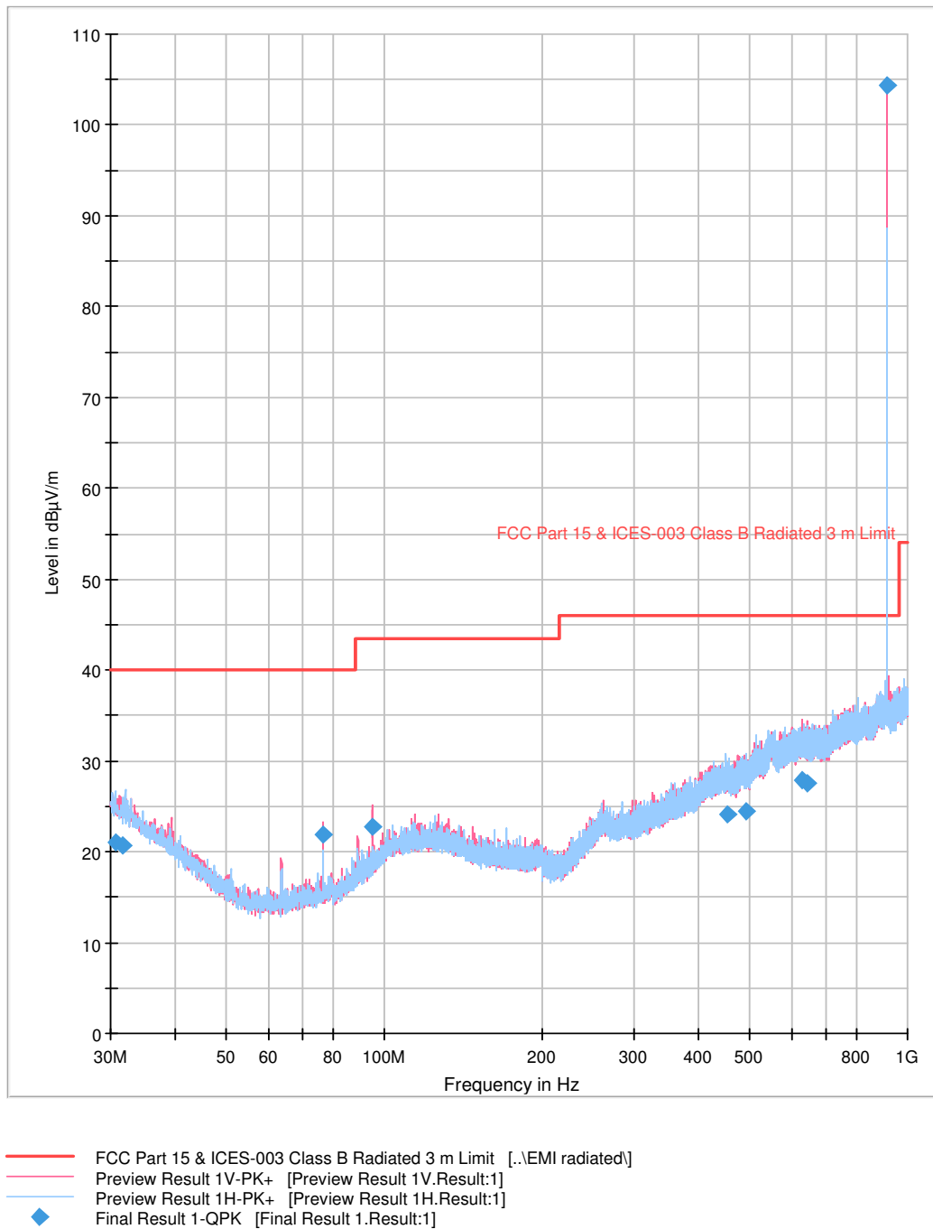
Figure 2.7.11-1 – 915 MHz Spurious Emissions Plot
