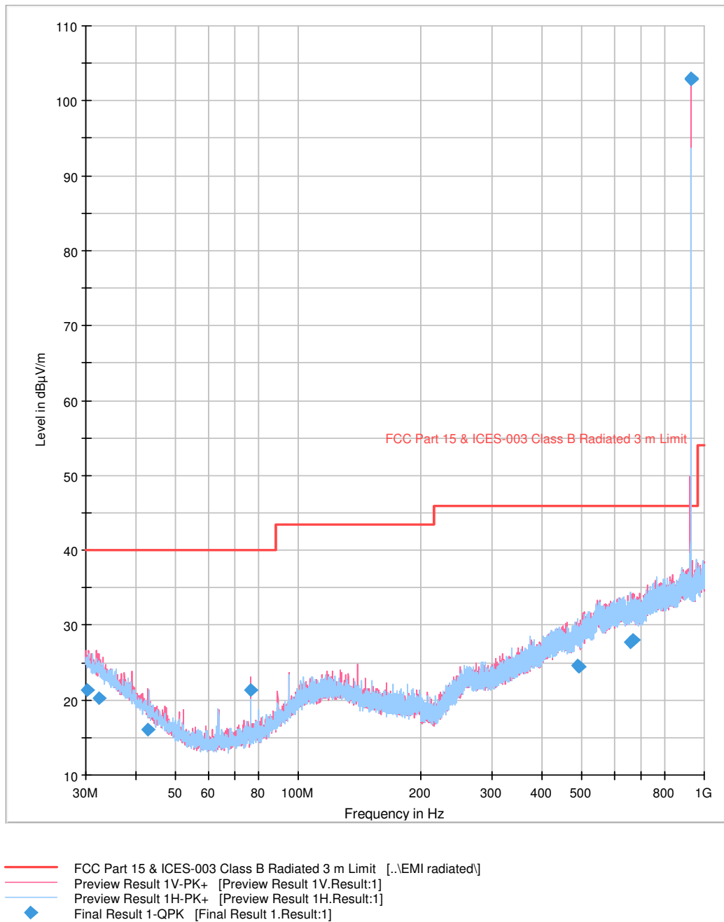
Figure 2.7.12-1 – 925 MHz Spurious Emissions Plot
