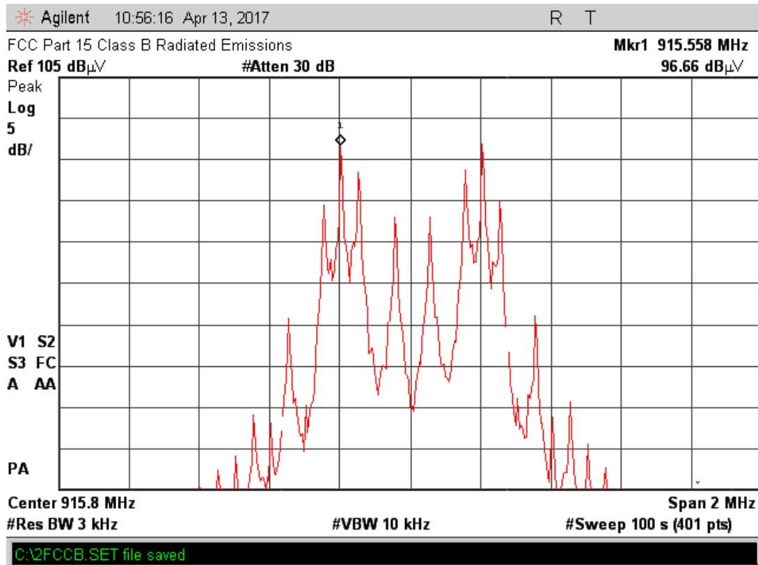
Figure 2.9.9-2 - Power Spectral Density – Mid Channel
