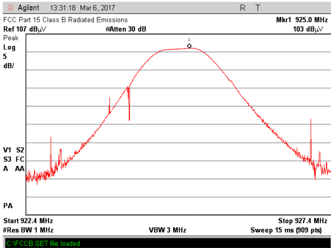
Figure 2.1.9-3 - High Channel Peak Power
