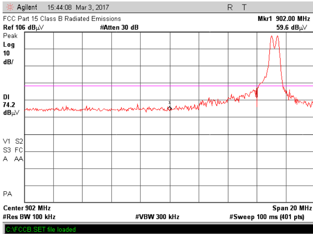
Figure 2.8.10-1 – Radiated Emissions Level at the Lower Band Edge Frequency
