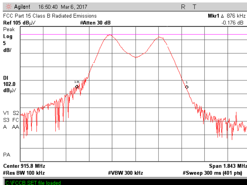
Figure 2.3.9-2 - Mid Channel Bandwidth
