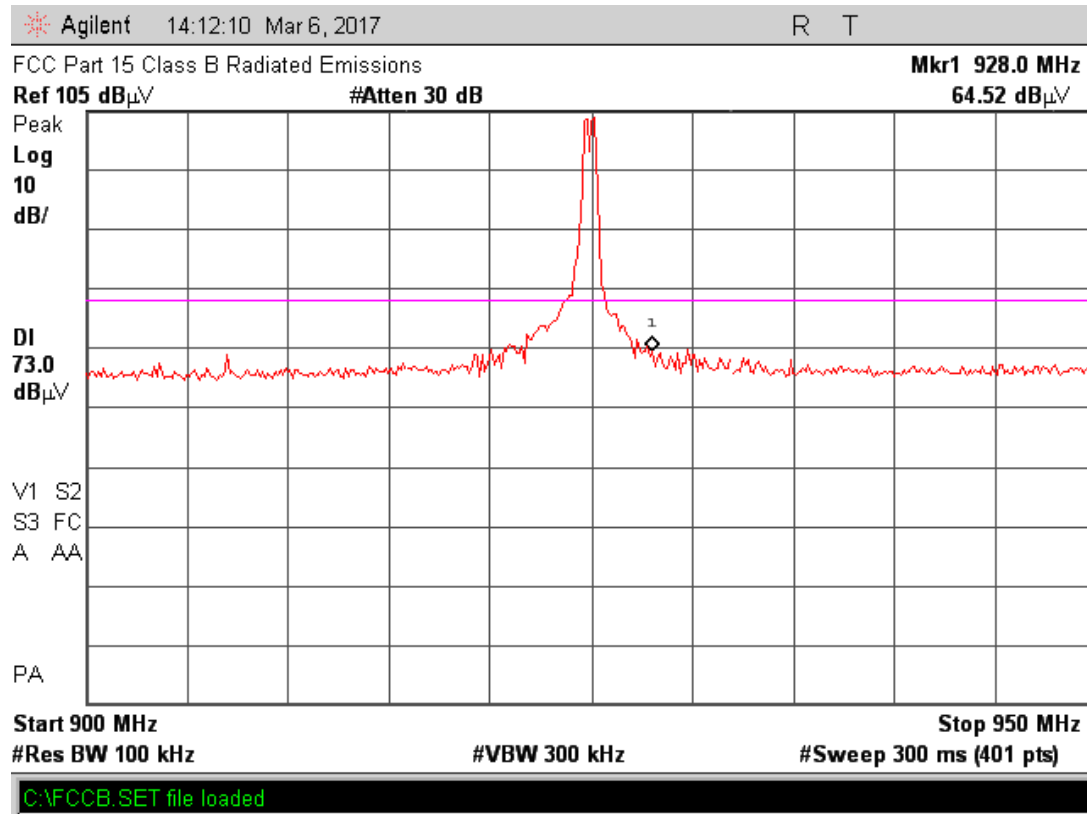
Figure 2.8.10-2 – Radiated Emissions Level at the Upper Band Edge Frequency
