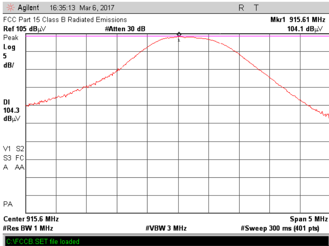
Figure 2.1.9-2 - Mid Channel Peak Power
