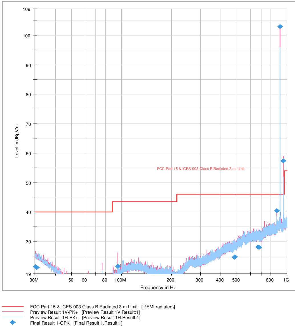
Figure 2.7.10-1 – 909 MHz Spurious Emissions Plot
