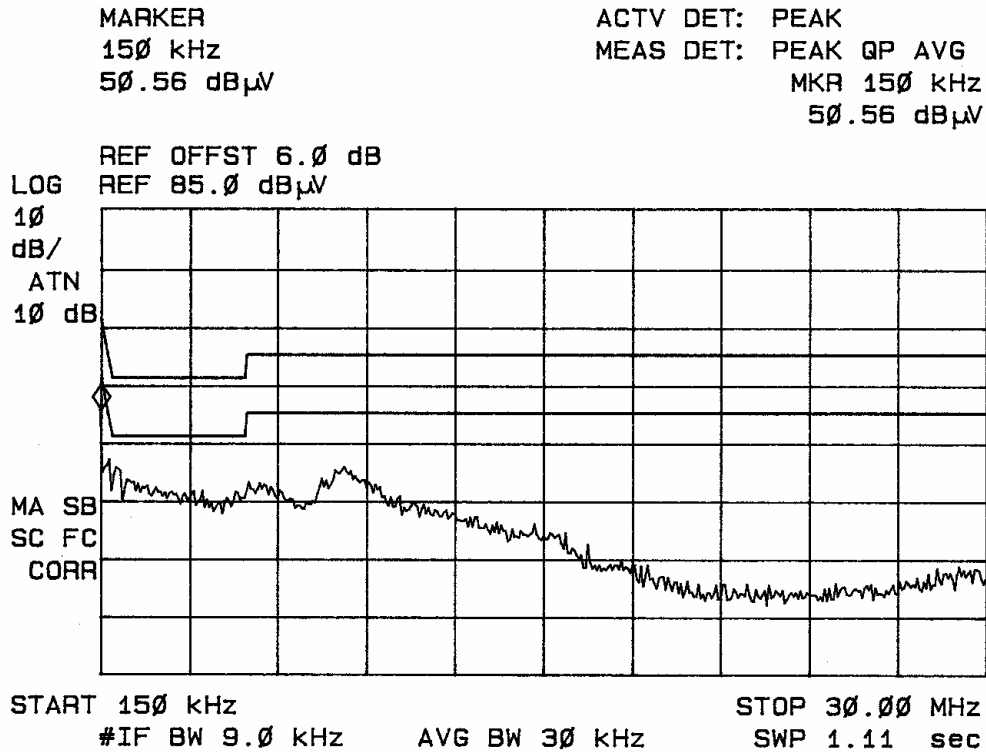
Figure one, Power Line Conducted Emissions Plot of Line 1.
