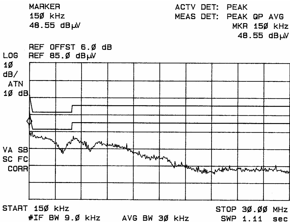
Figure two, Power Line Conducted Emissions Plot of Line 2.
