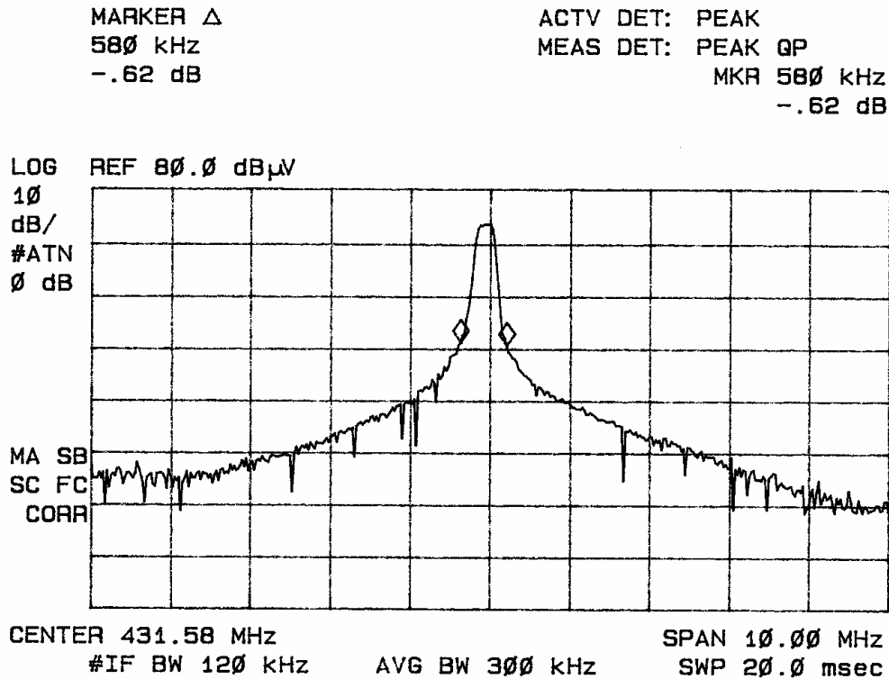
Figure seven occupied bandwidth emissions taken at 1 meter in screen room.
