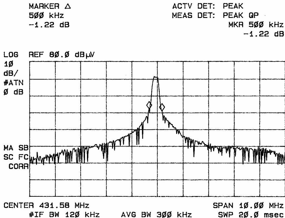
Figure five occupied bandwidth emissions taken at 1 meter in screen room.
