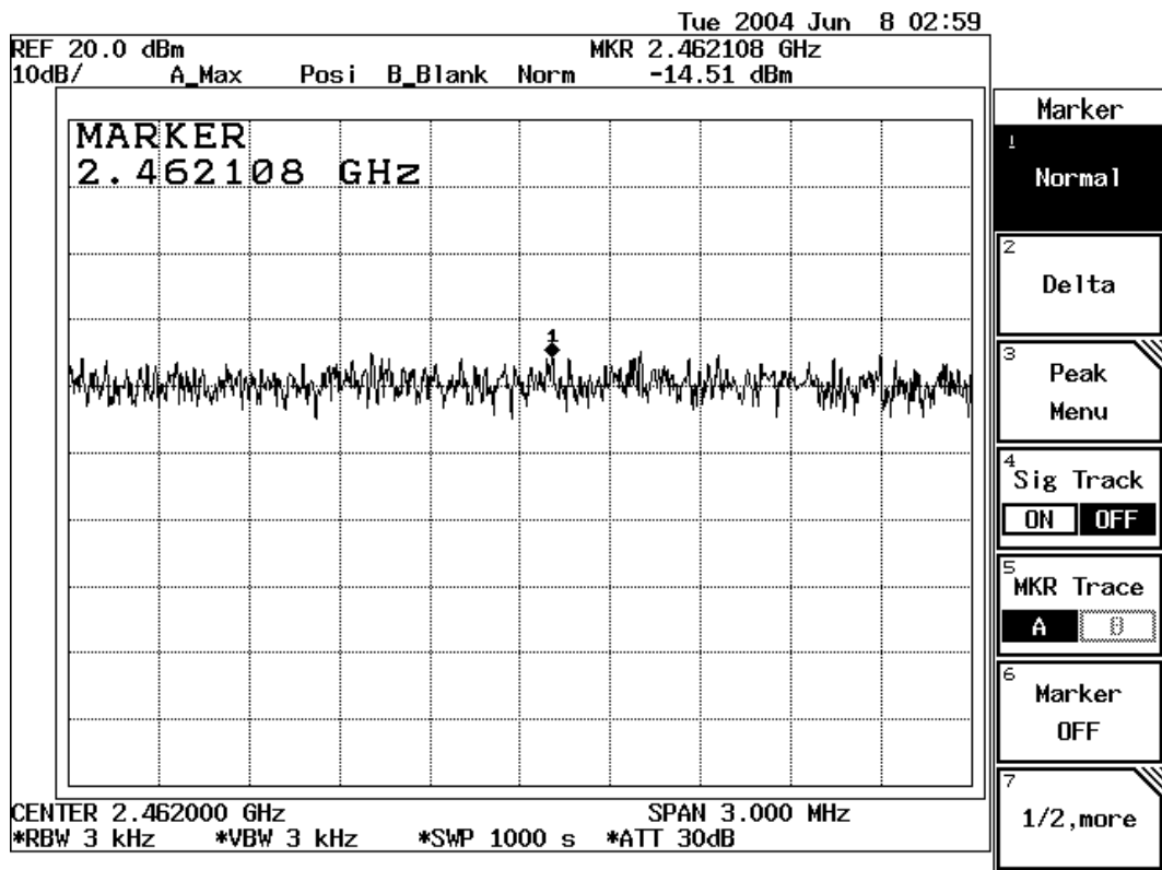
Figure Channel 11: 11Mbps
