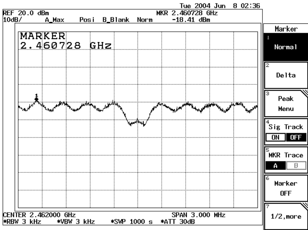
Figure Channel 11: 54Mbps
