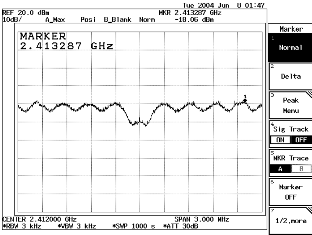
Figure Channel 1: 54Mbps
