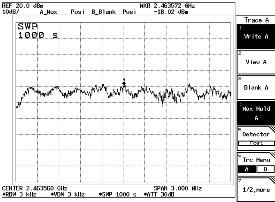
Figure Channel 11: 54Mbps
