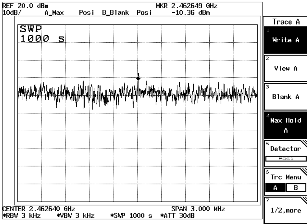
Figure Channel 11: 11Mbps
