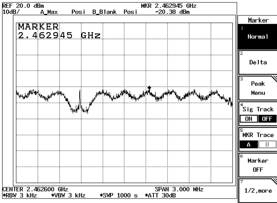
Figure Channel 11: 54Mbps
