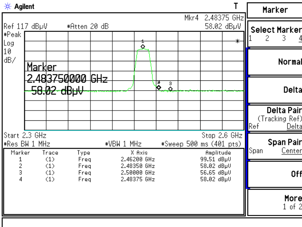
Figure Channel 11: (Vertical)
