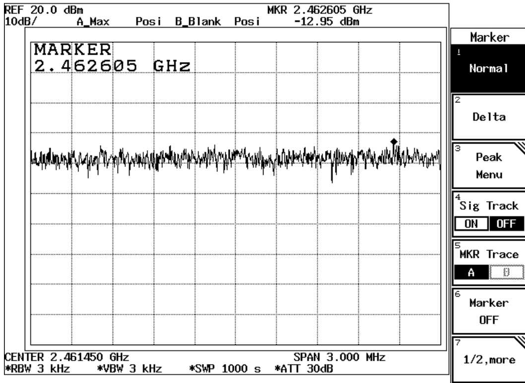
Figure Channel 11: 11Mbps
