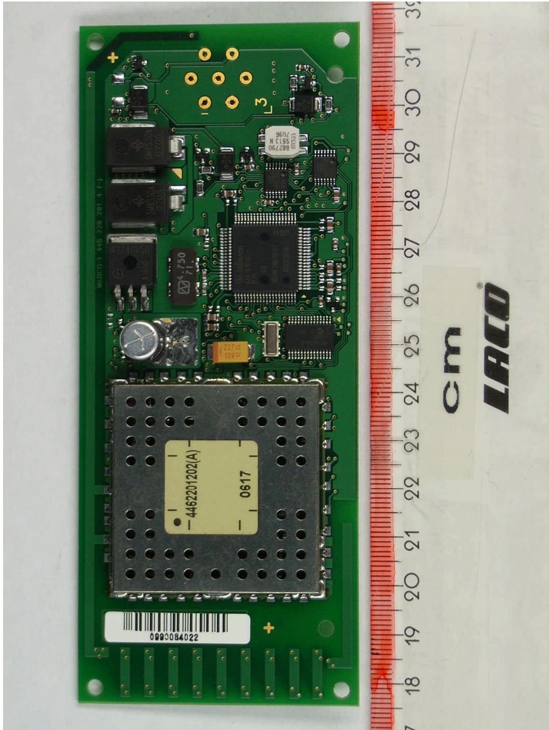
71209eut8.JPG IVTM ECU, pcb top view with shielding
