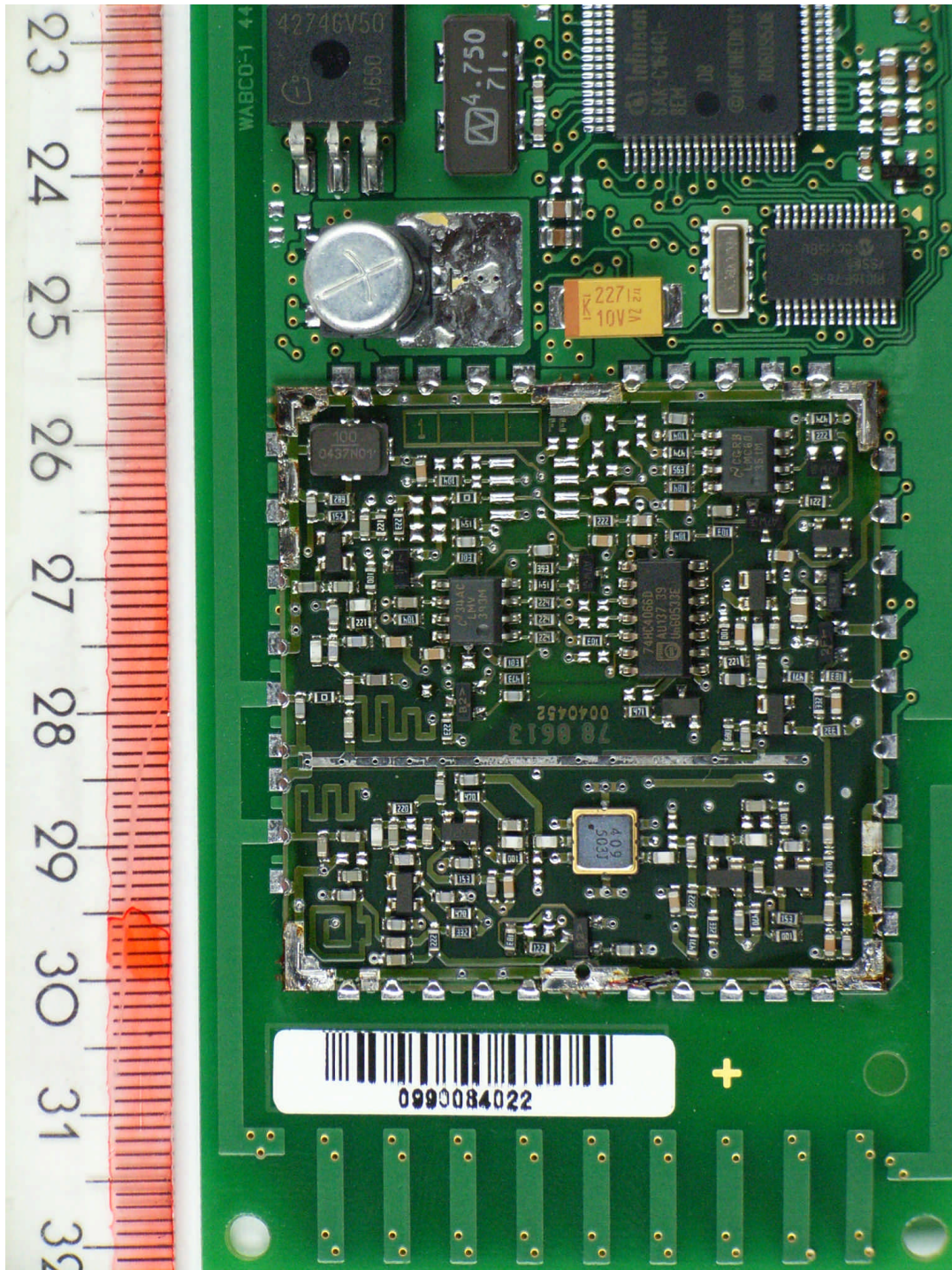
71209eut3.JPG IVTM ECU, detail view radio board without shielding
