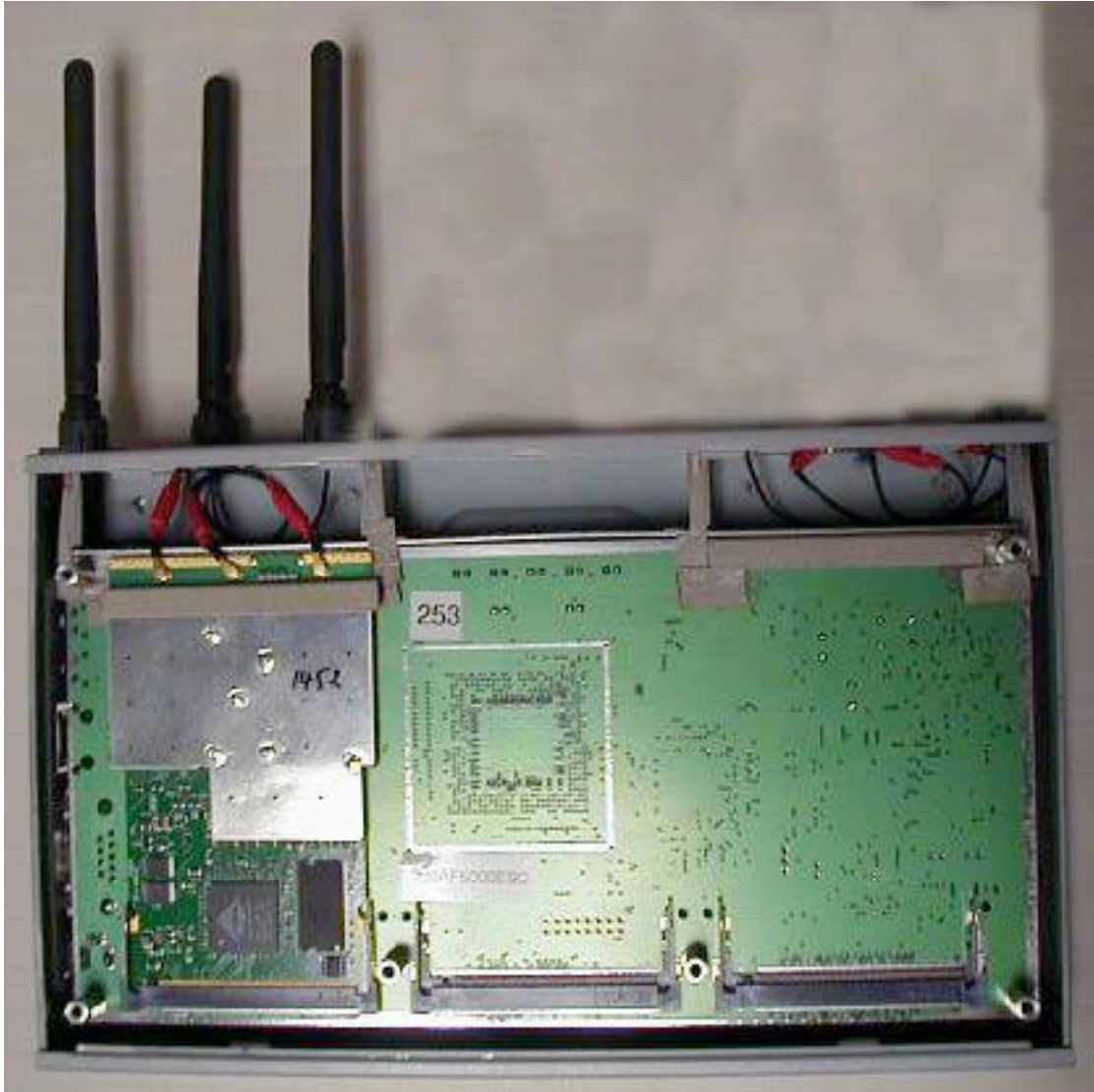
Airgo True MIMO AP Internal Photographs FCC ID: SA3-AGN1201AP0000
