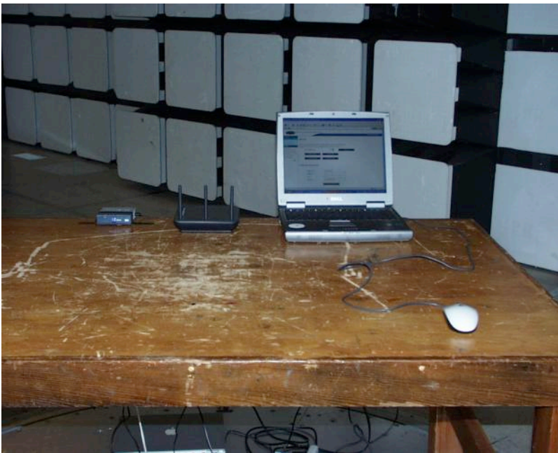
Radiated emissions
