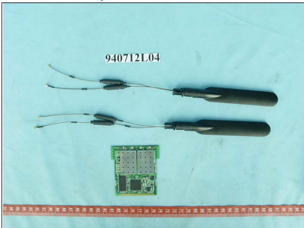
Dipole antenna with test mode 2
