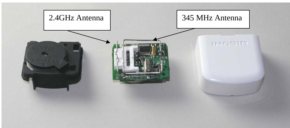
Bottom View PCBA w/Antenna Assembly
