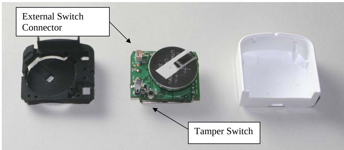
Top View PCBA
