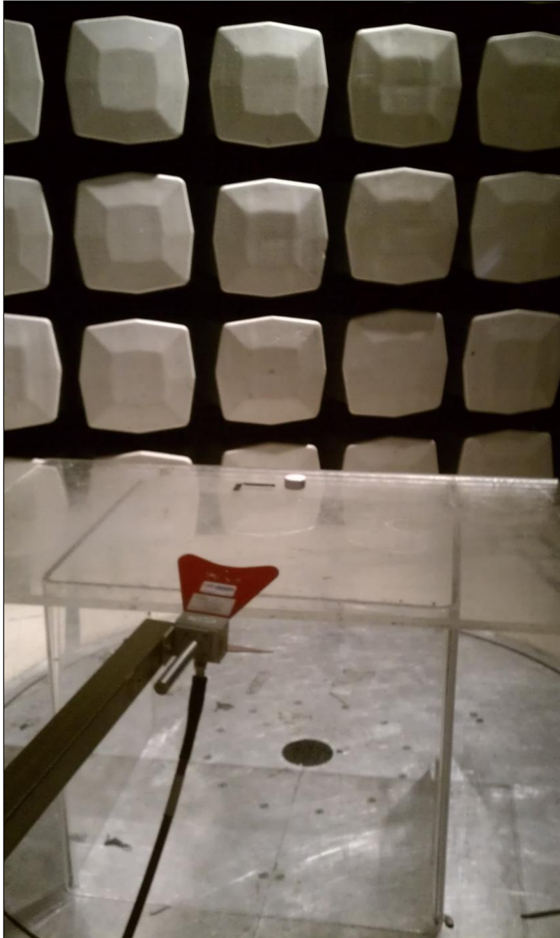
Photograph 3. Radiated Spurious Emissions, Test Setup, 1 GHz – 4 GHz
