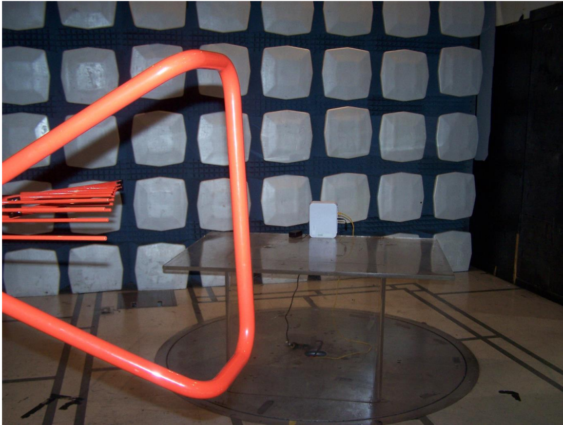
Photograph 4. Radiated Spurious Emissions, Test Setup
