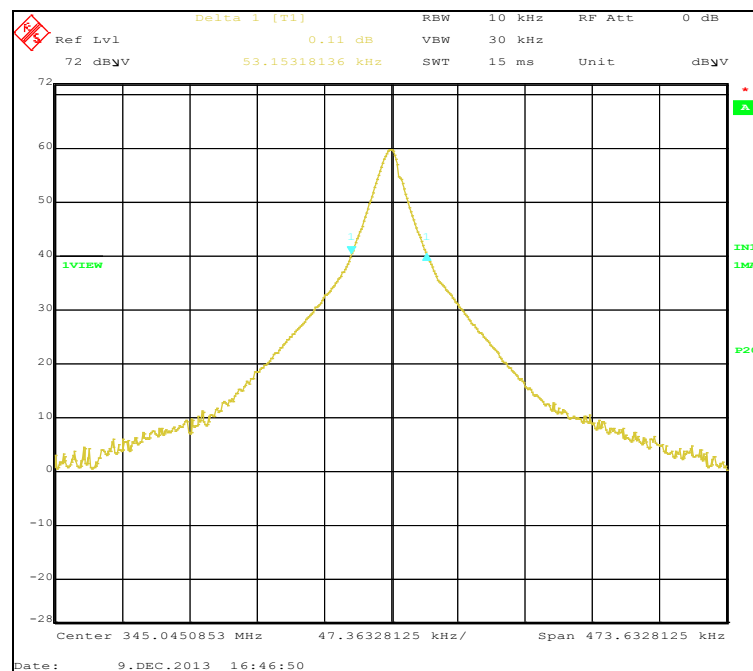
Plot 11. 20 dB Bandwidth Plot
