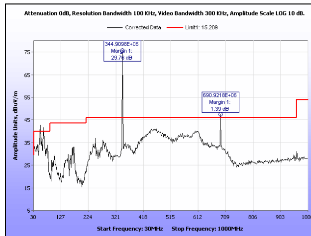
Plot 8. Radiated Spurious Emissions, 30 MHz – 1 GHz
