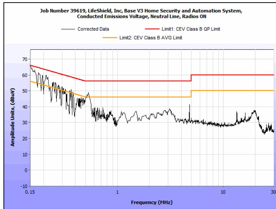
Plot 6. Conducted Emissions, 15.207(a), Neutral Line (Pre-scans performed with a Peak detector)
