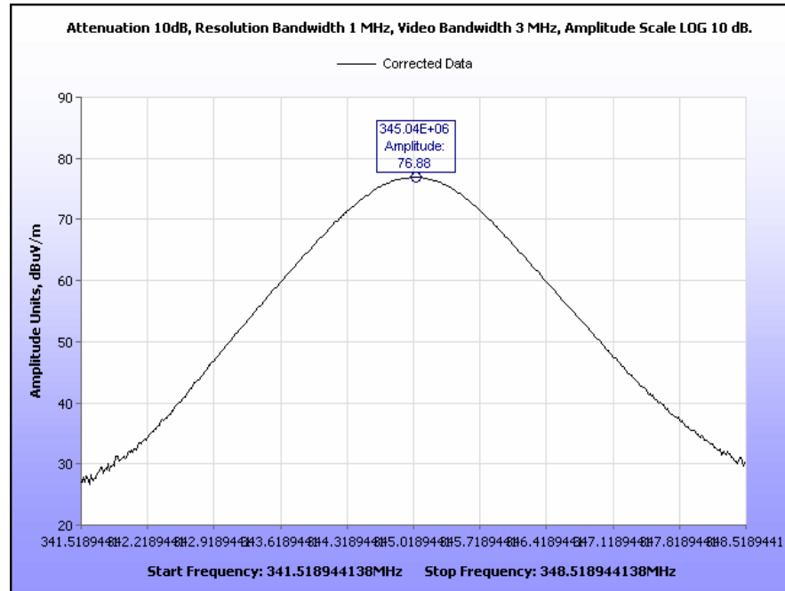
Plot 7. Field Strength of Fundamental, 345 MHz, Peak, with Duty Cycle Corrected
