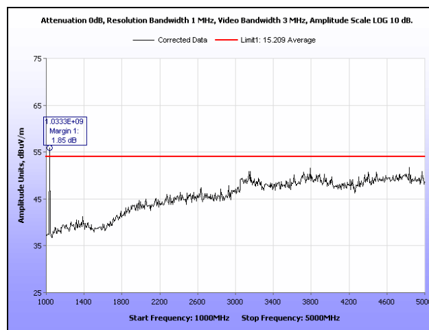
Plot 9. Radiated Spurious Emissions, 1 GHz – 5 GHz, Peak under Average
