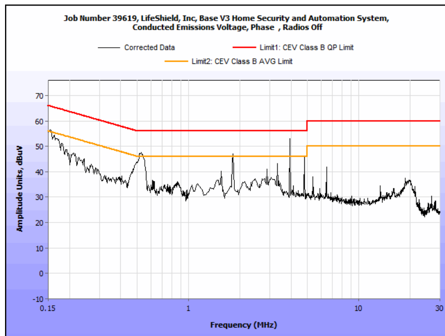
Plot 1. Conducted Emission, Phase Line Plot (Pre-scans performed with a Peak detector)
