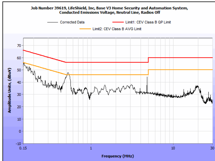
Plot 2. Conducted Emission, Neutral Line Plot (Pre-scans performed with a Peak detector)
