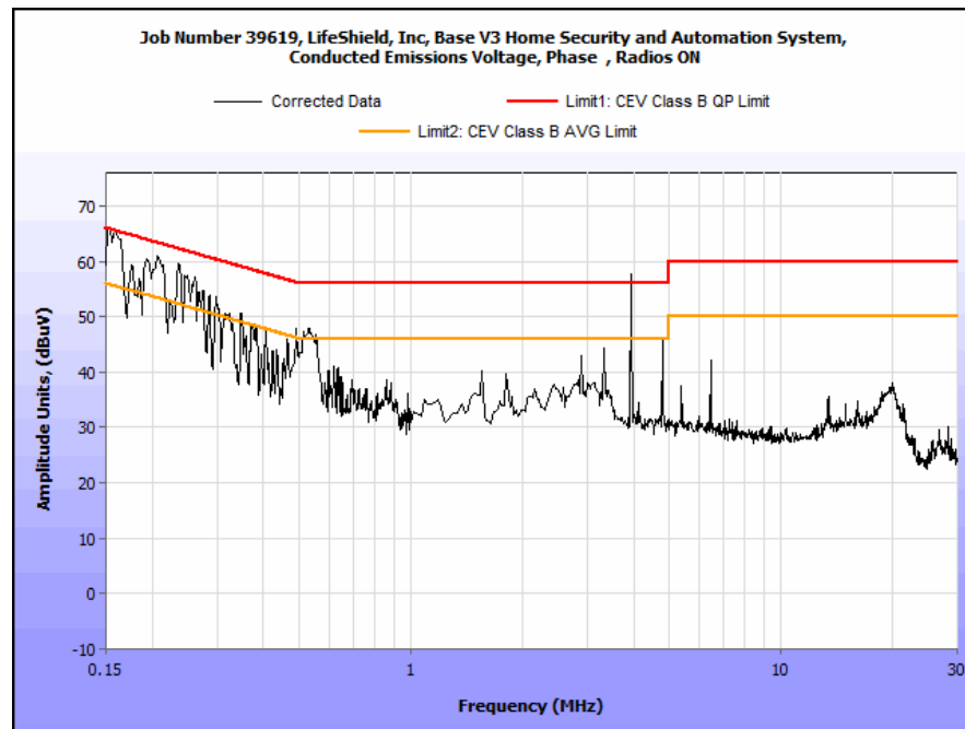
Plot 5. Conducted Emissions, 15.207(a), Phase Line (Pre-scans performed with a Peak detector)
