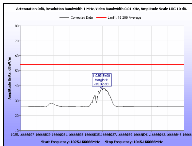
Plot 10. Radiated Spurious Emissions, 1 GHz – 5 GHz, 1033 MHz
