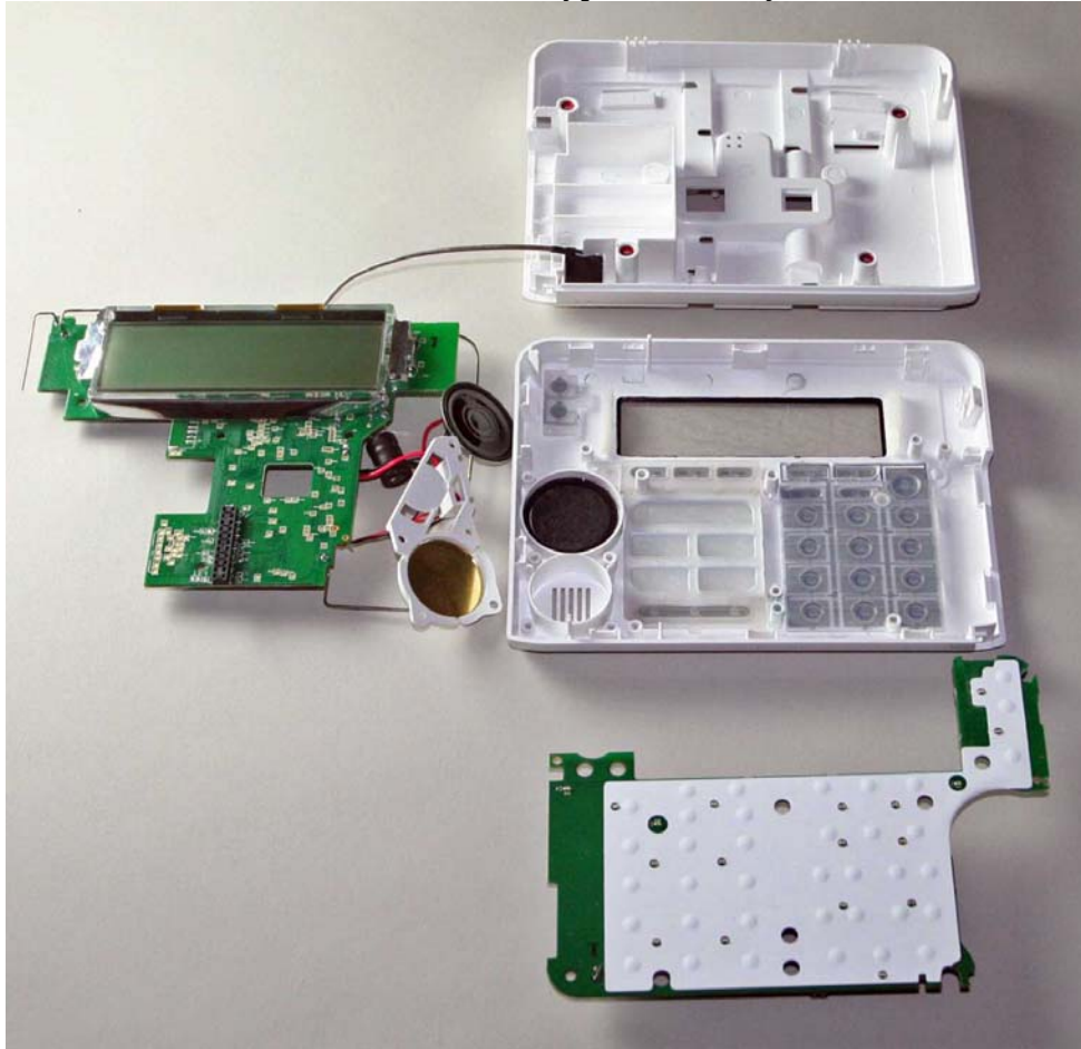
PCB/Antenna/Keypad Assembly
