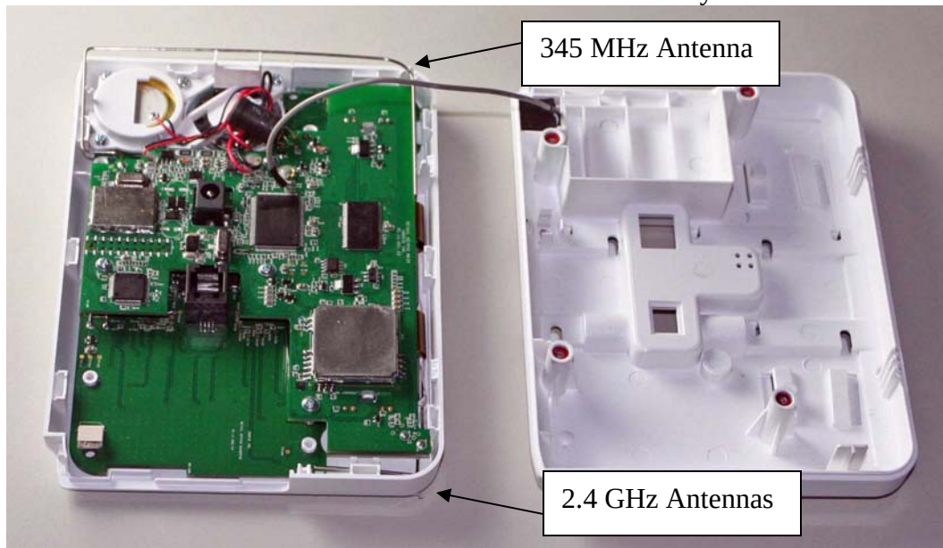
Bottom View PCB w/Antenna Assembly
