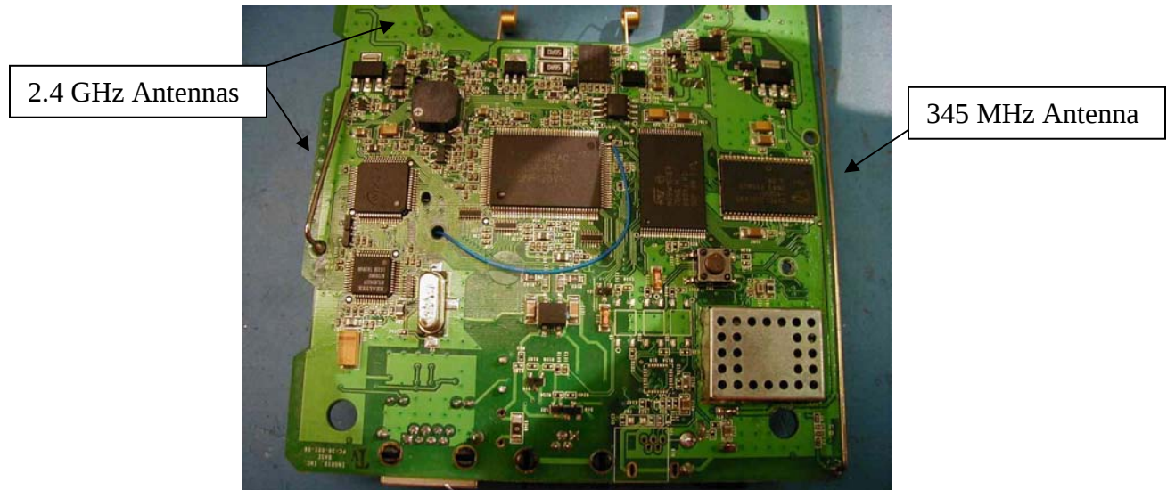
PCB/Antenna/ Assembly Side 1
