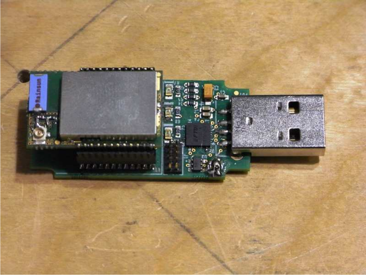
SPZB32W1A2.1 + demo board
