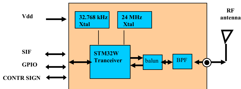
Figure 2. SPZB32W1C2.1 Block diagram
