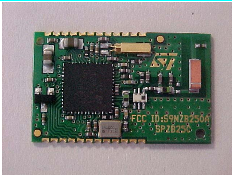
Radio module with MURATA antenna
