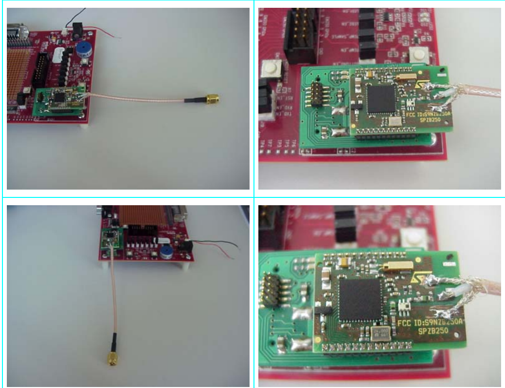
Radio module + antenna connector (for conducted spurious test)
