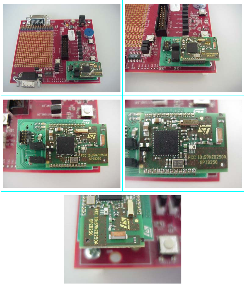
Equipment under test identification: Test jig + Radio module
