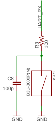
Push Button
