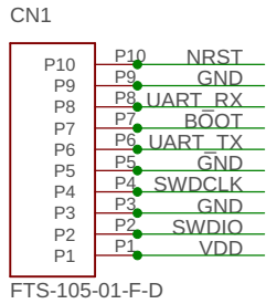
ARM10 Debug Connector
