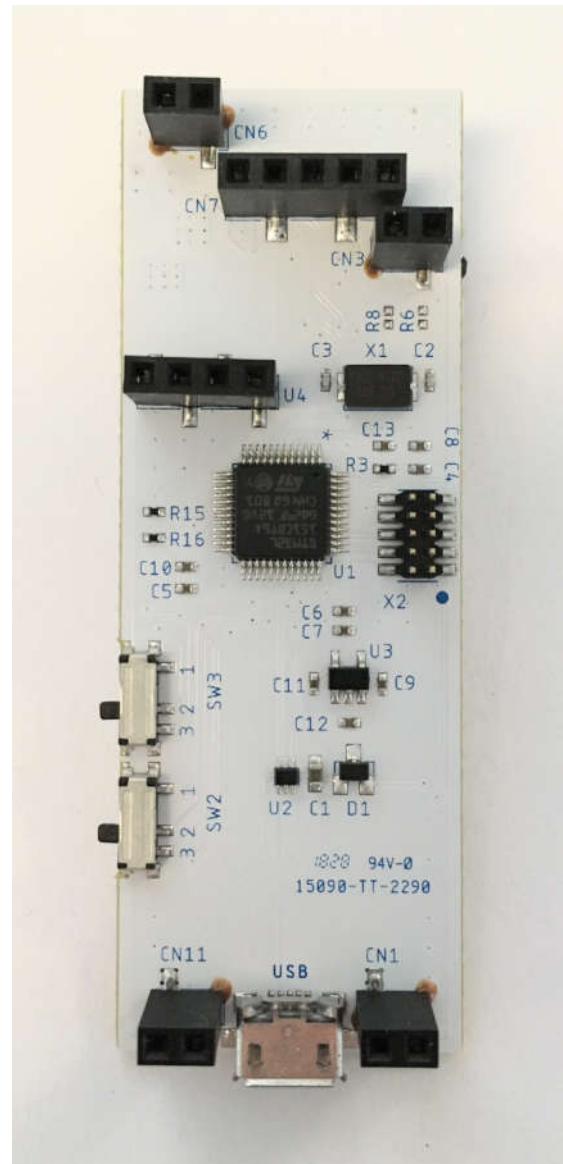
Figure 8: STEVAL-BCN002v1D bottom view
