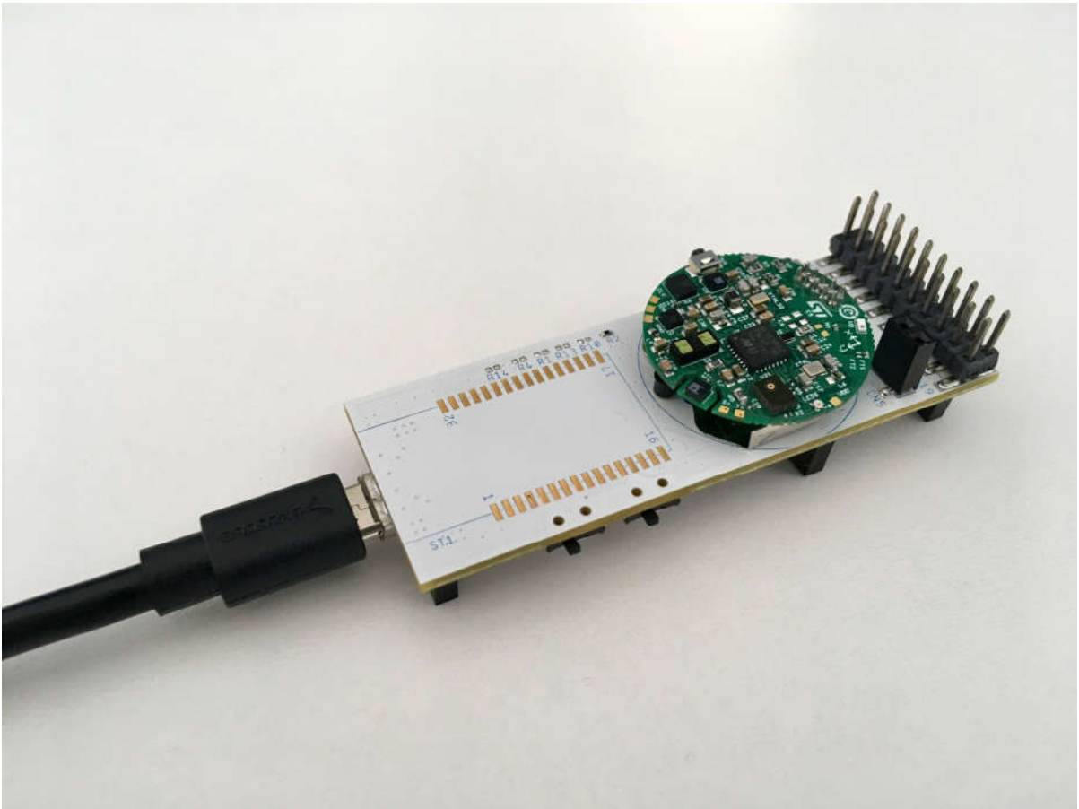
Figure 1: STEVAL-BCN002v1B (STEVAL-BCN002v1 + STEVAL-BCN002v1D) with USB cable
