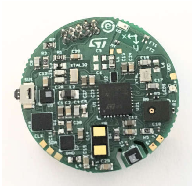
Figure 2: STEVAL-BCN002v1 Top view
