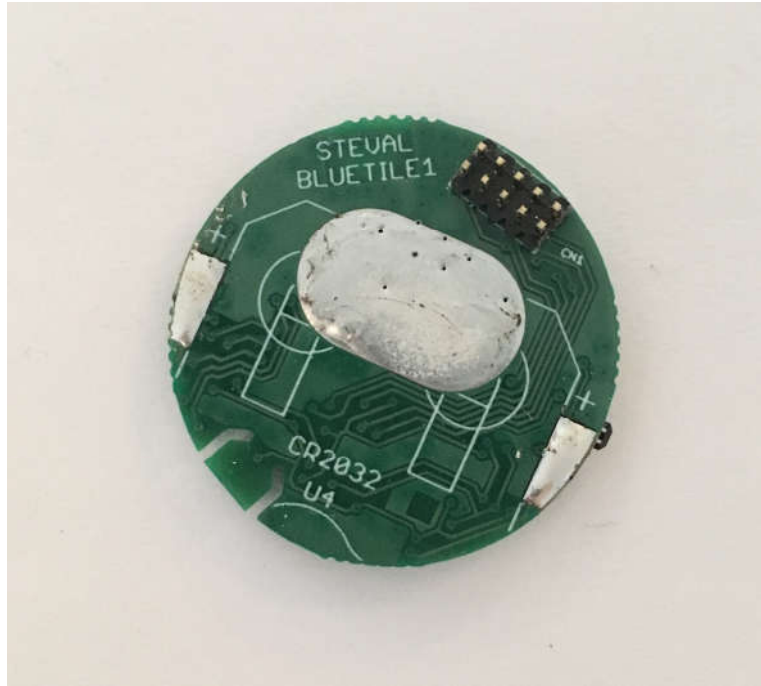
Figure 4: STEVAL-BCN002v1 bottom view without battery holder
