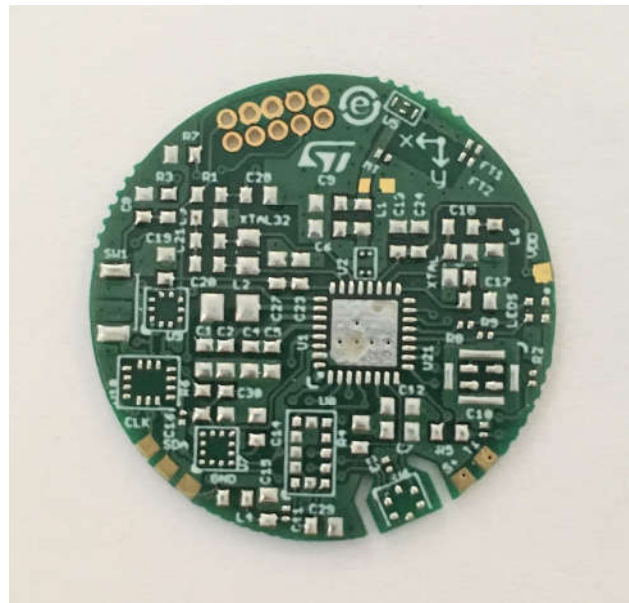
Figure 3: STEVAL-BCN002v1 top view without components
