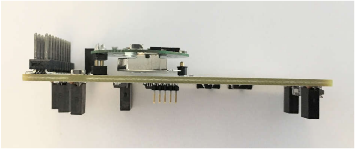
Figure 10: STEVAL-BCN002v1B side view
