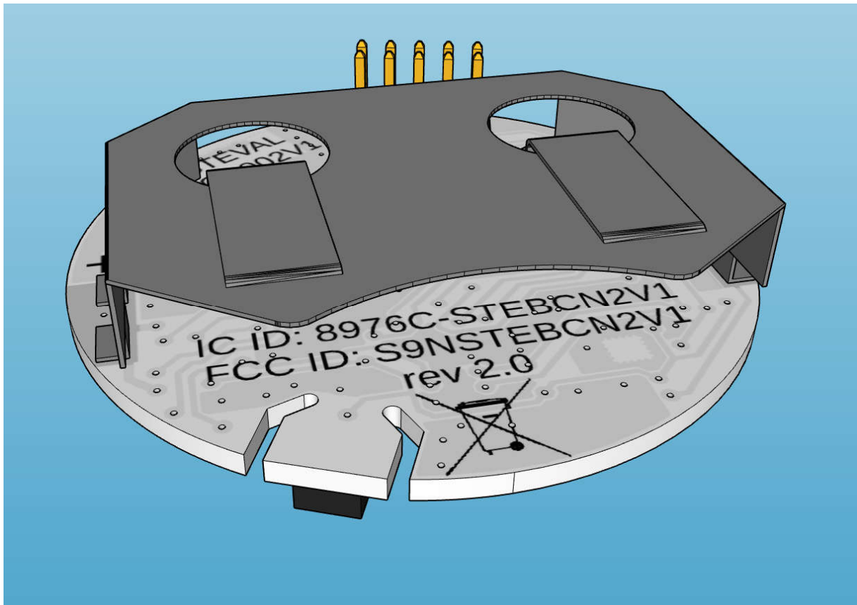
Figure 1: STEVAL-BCN002V1 bottom view with battery holder
