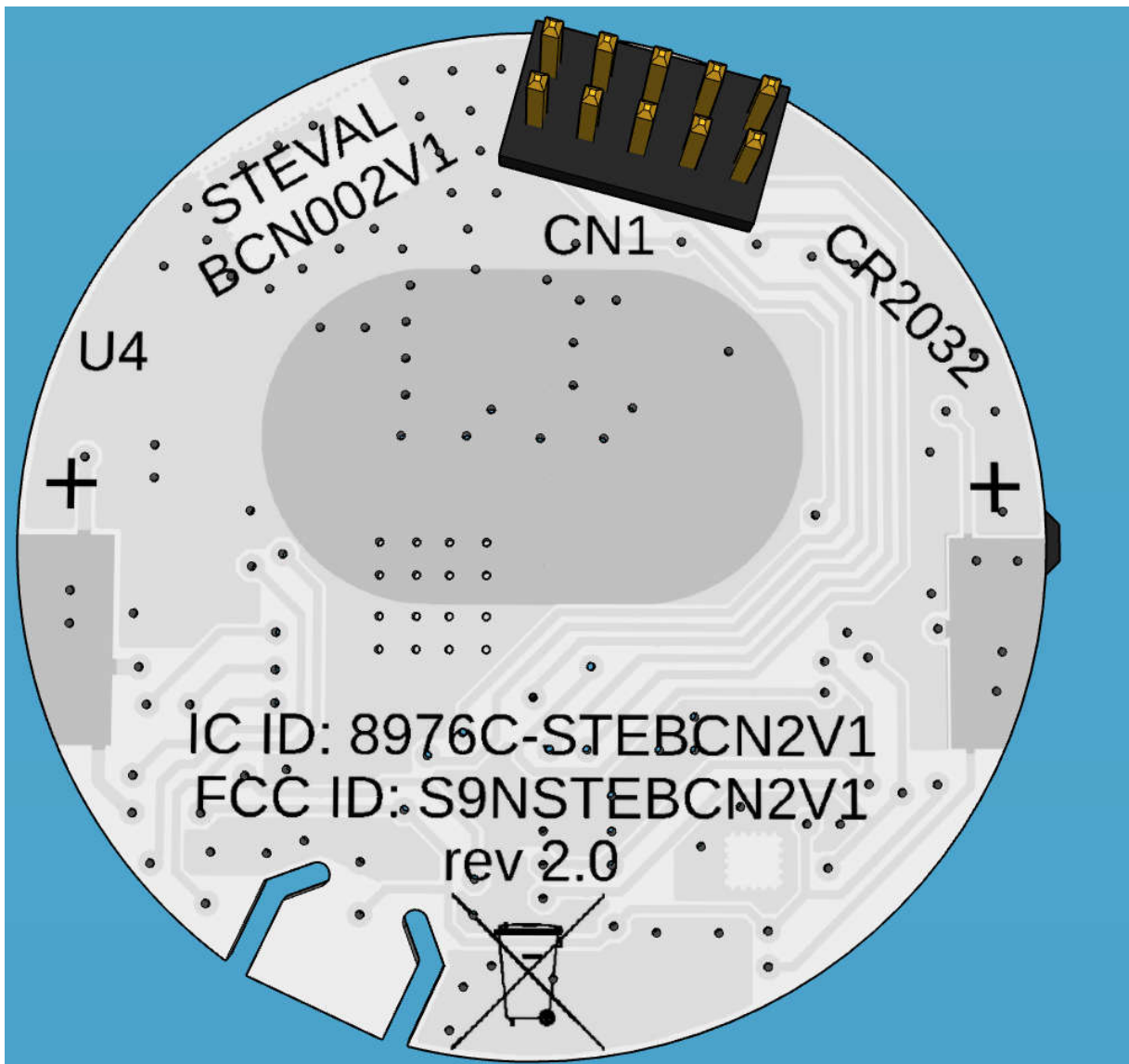
Figure 2: STEVAL-BCN002V1 bottom view without battery holder
