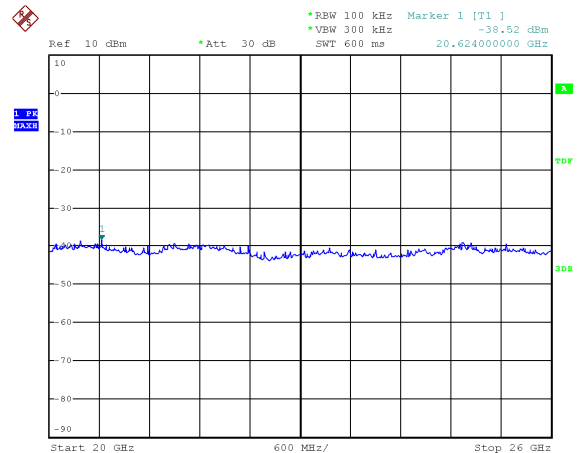
Plot 6 (20÷26GHz)
