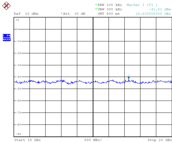
Plot 5 (15÷20GHz)
