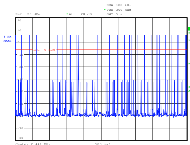
Plot 4 (DH3 packet) – N° of packets in 5s. (28 hops)
