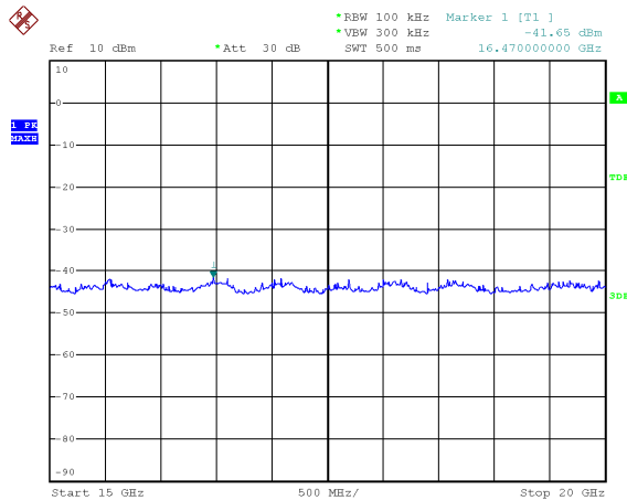
Plot 5 (15÷20GHz)
