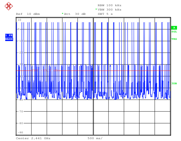
Plot 2 (DH1 packet) – N° of packets in 5s. (50 hops)
