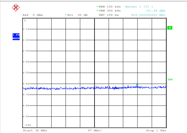
Plot 1 (30÷1000MHz)
