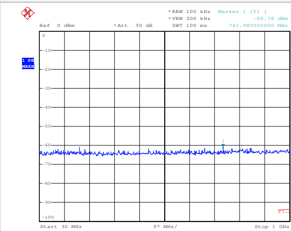
Plot 1 (30÷1000MHz)
