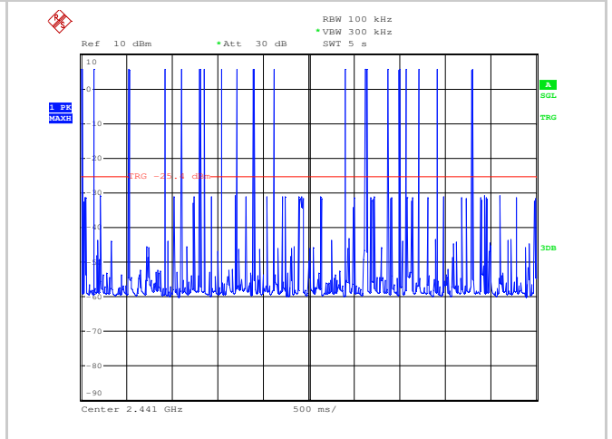
Plot 6 (DH5 packet) – N° of packets in 5s. (19 hops)
