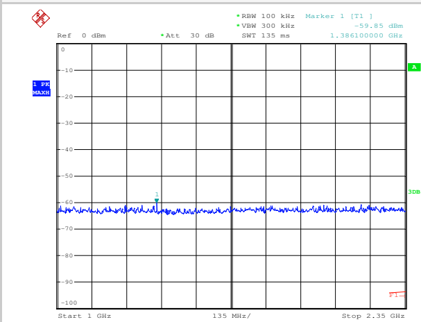
Plot 2 (1÷2.35GHz)
