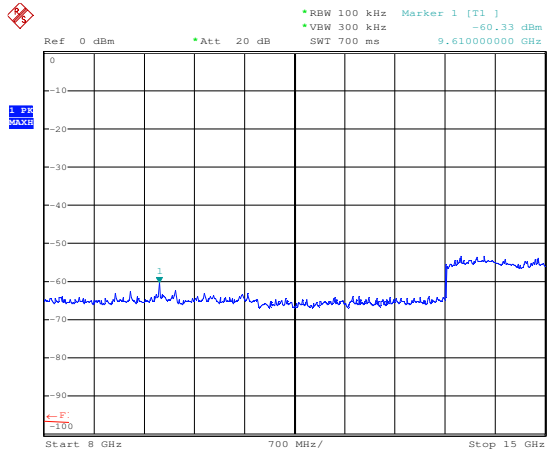
Plot 5 (8÷15GHz)
