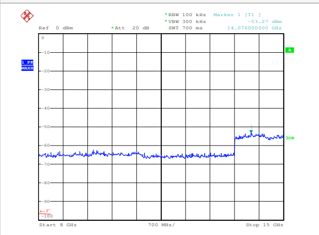
Plot 5 (8÷15GHz)
