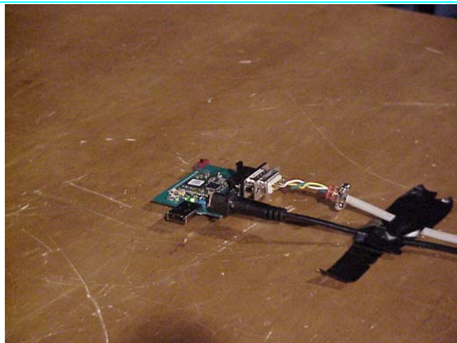
Set up of Radiated emission test
