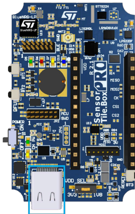
Figure 15. Power components - top view
