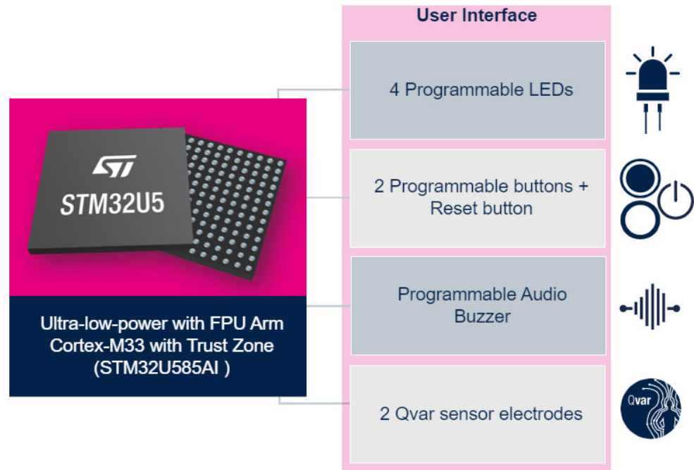
Figure 17. SensorTile.box PRO user interface
