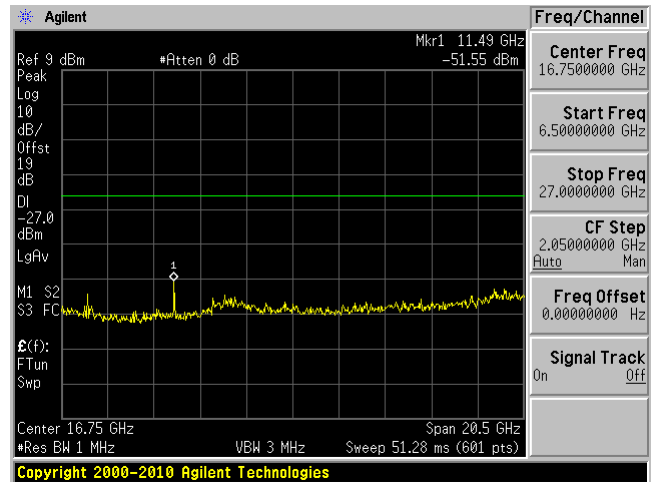
Low Channel Chain 2: 6.5 GHz- 27 GHz
