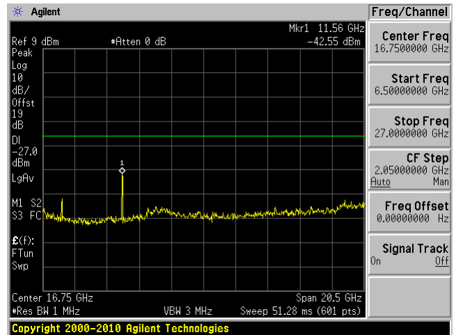
Middle Channel Chain 1: 6.5 GHz- 27 GHz
