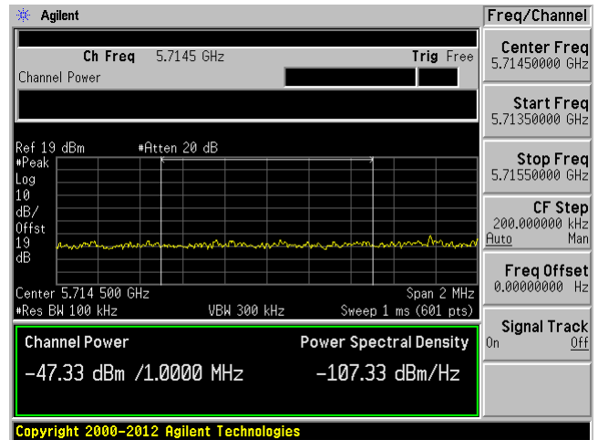
Low Channel Chain 0 (-27 dBm limit)
