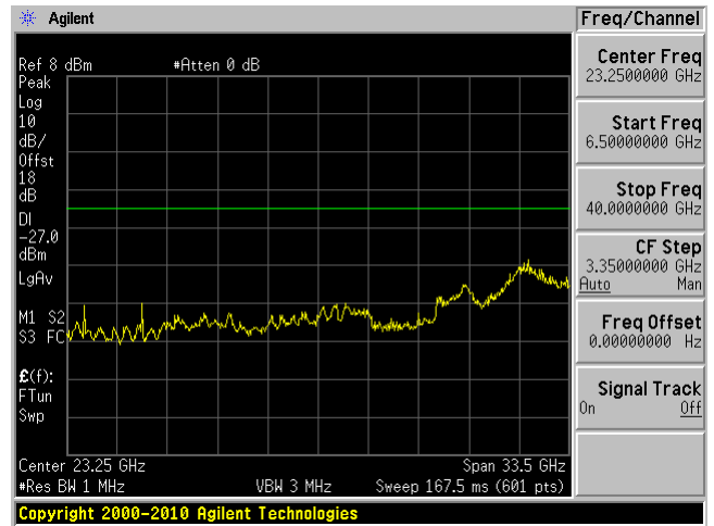
Low Channel Chain 2: 6.5 GHz- 40 GHz
