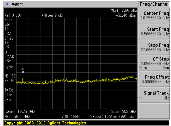
Low Channel Chain 0: 6.5 GHz- 27 GHz
