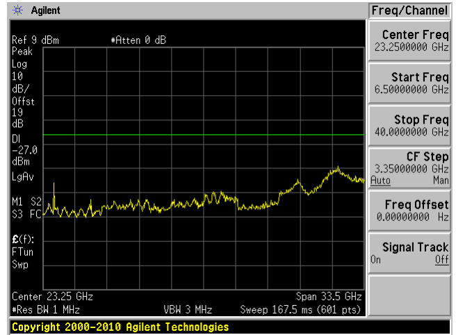
Low Channel Chain 0: 6.5 GHz- 40 GHz
