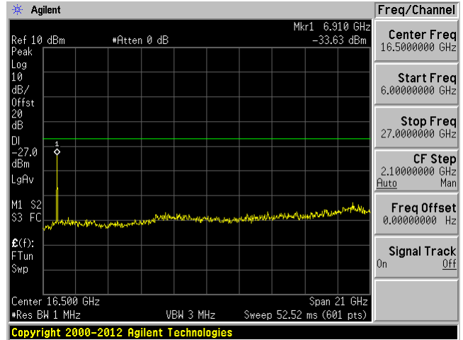
Low Channel Chain 0: 6 GHz- 27 GHz
