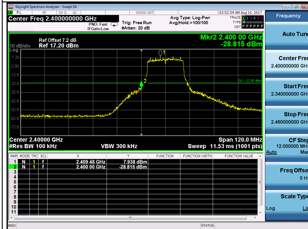
802.11n-HT20-2412MHz Chain 1
