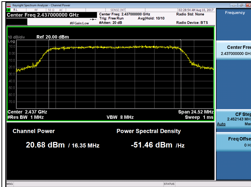
802.11g-2437MHz Chain 0
