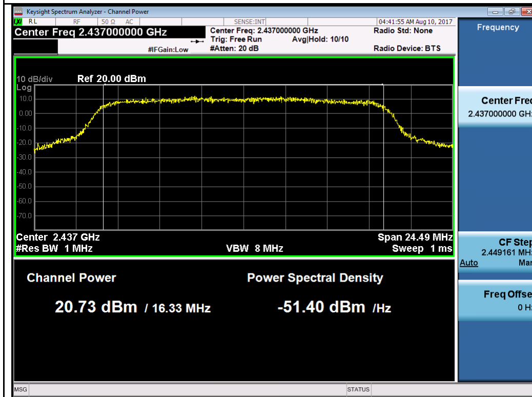
802.11g-2437MHz Chain 3
