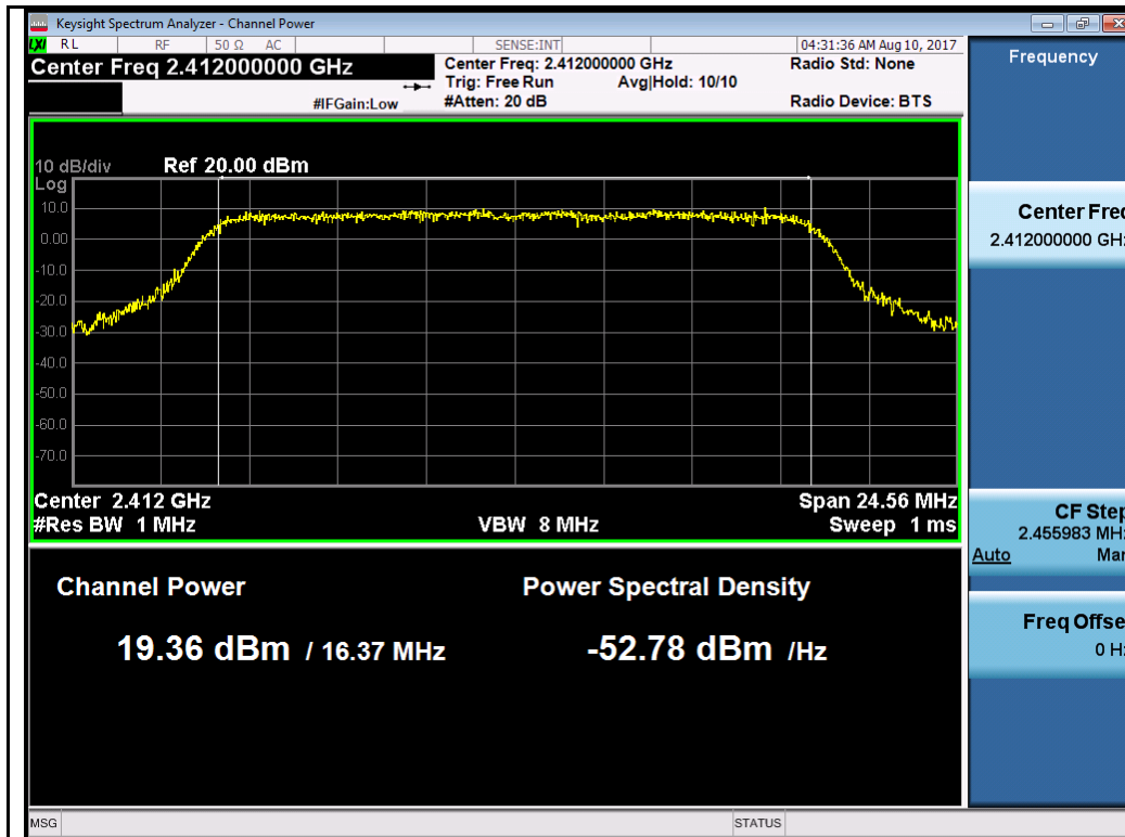
802.11g-2412MHz Chain 2
