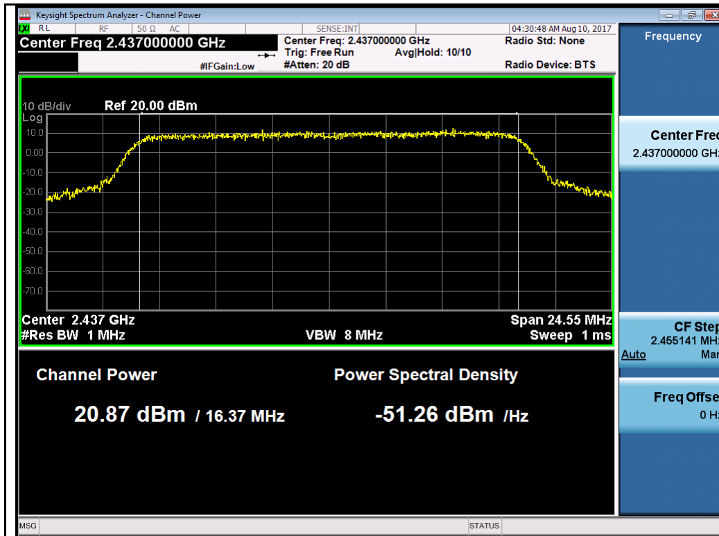
802.11g-2437MHz Chain 2
