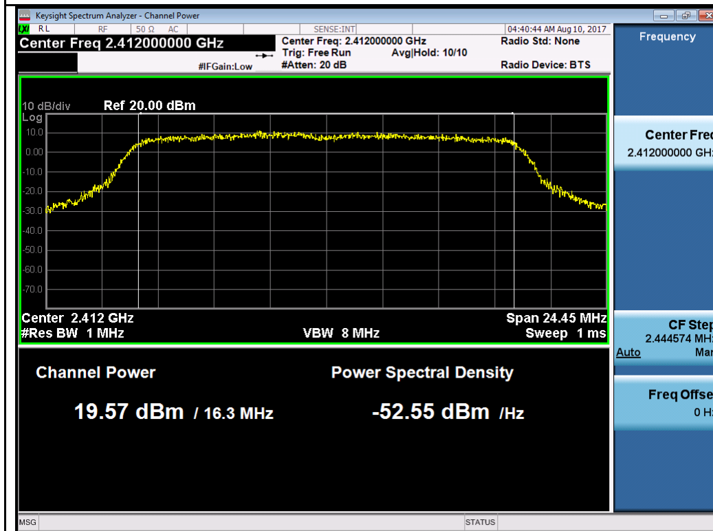
802.11g-2412MHz Chain 3
