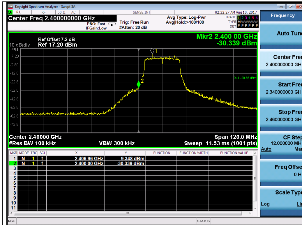
802.11n-HT20-2412MHz Chain 0
