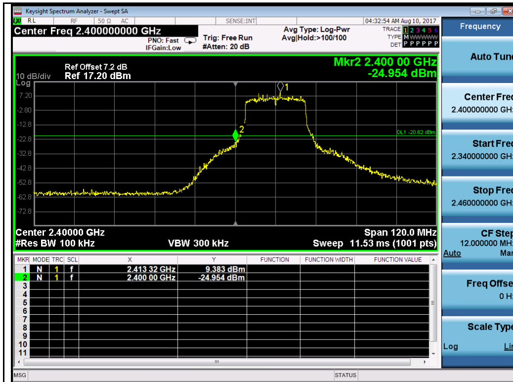
802.11n-HT20-2412MHz Chain 2
