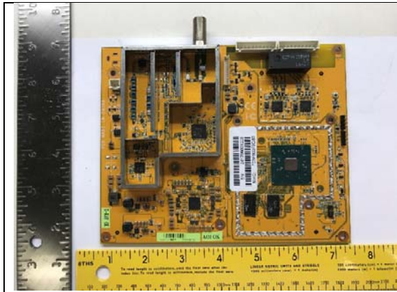
Cable Modem - Top View
