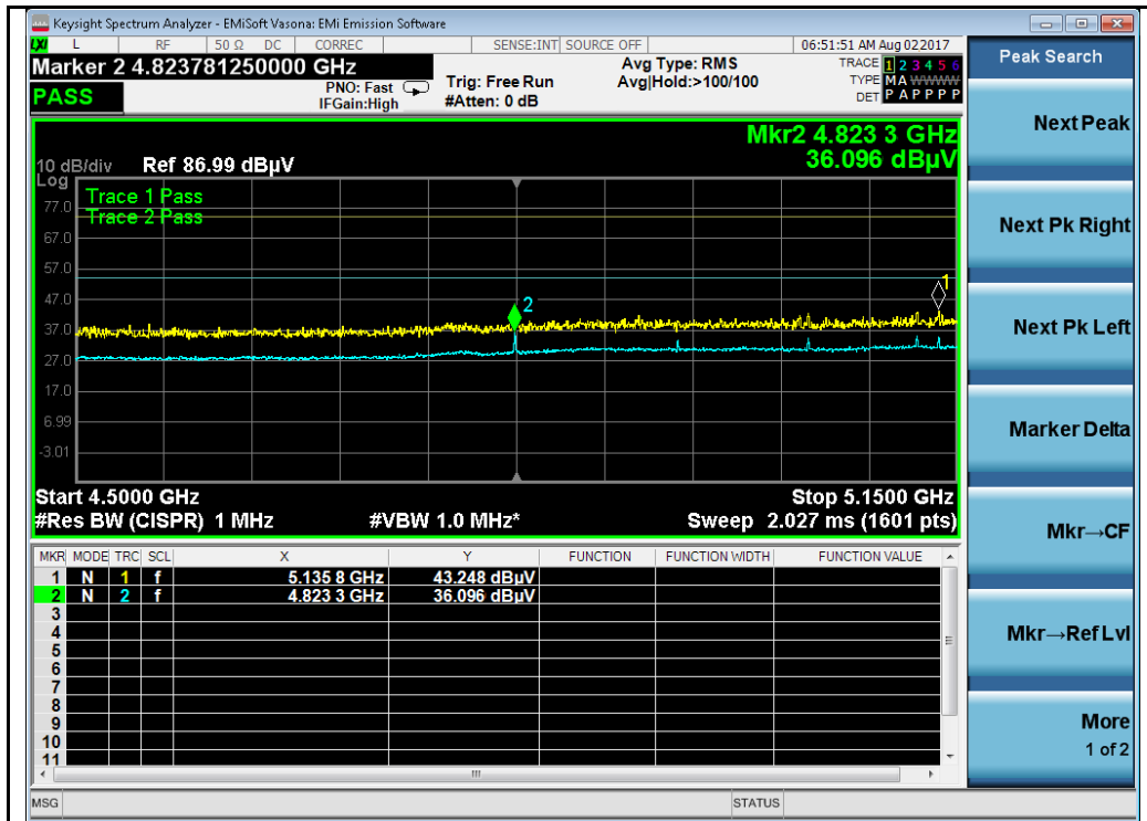
802.11a-5180MHz
