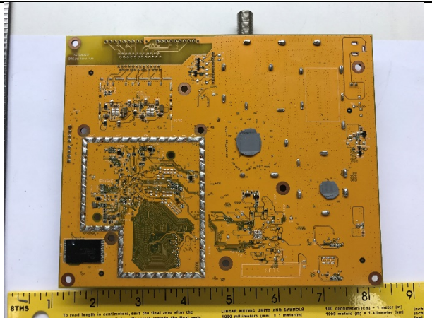
Cable Modem - Bottom View
