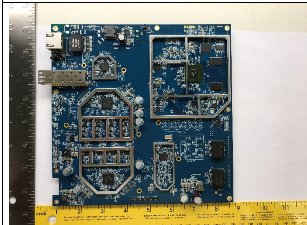
AP Board - Top View
