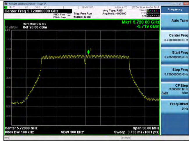
PSD-802.11n-20M-CROSS-5720M-chain2
