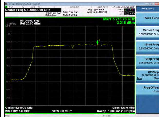
PSD-802.11ac-CROSS-5690M-chain1
