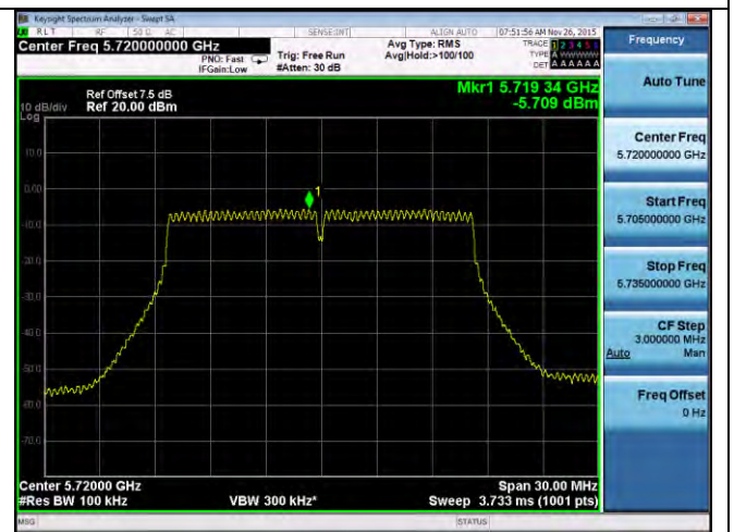
PSD-802.11a-CROSS-5720M-chain2
