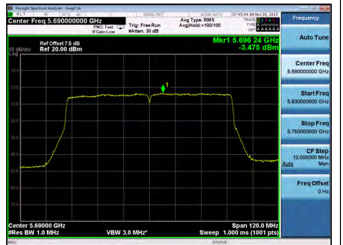
PSD-802.11ac-CROSS-5690M-chain2
