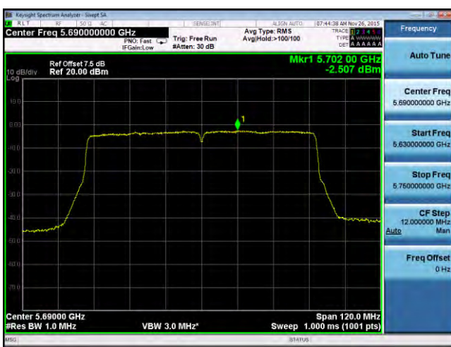
PSD-802.11ac-CROSS-5690M-chain3
