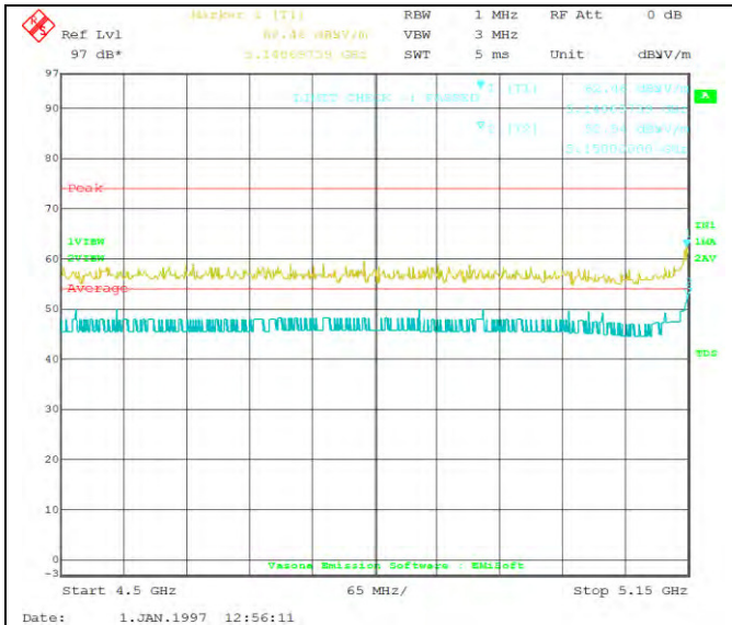
802.11n-HT40 5190M
