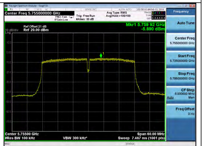
PSD-802.11n-40M-5755M-chain4
