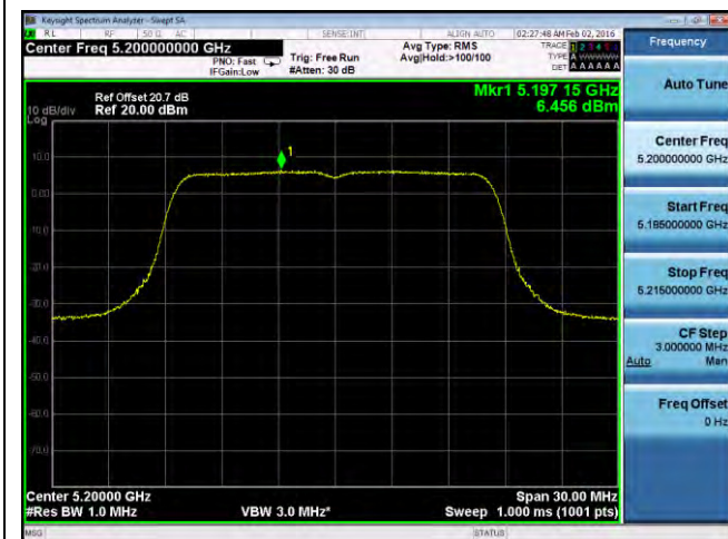
PSD-802.11a-5200M-chain1
