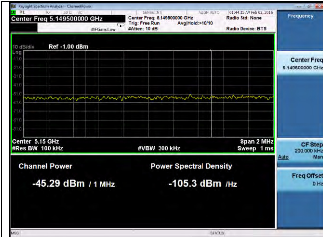
Band Edge-802.11a-5180M-chain1
