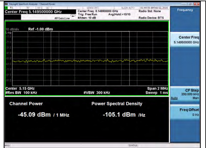
Band Edge-802.11a-5180M-chain2
