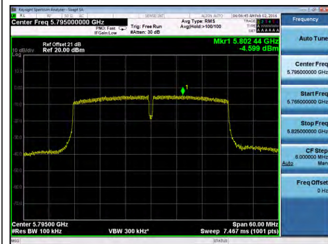
PSD-802.11n-40M-5795M-chain1
