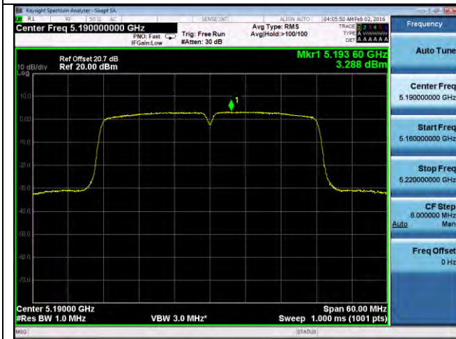
PSD-802.11n-40M-5190M-chain3
