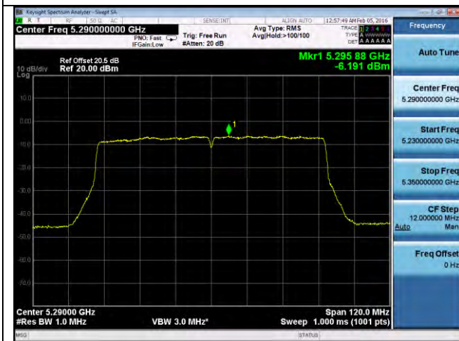
PSD-802.11ac-80M-5290M-chain1
