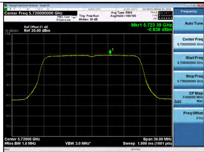
PSD-802.11n-20M-CROSS-5720M-chain2
