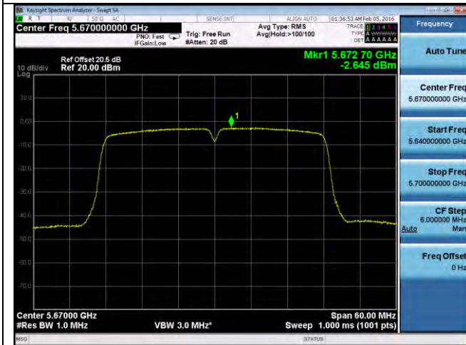
PSD-802.11n-40M-5670M-chain1
