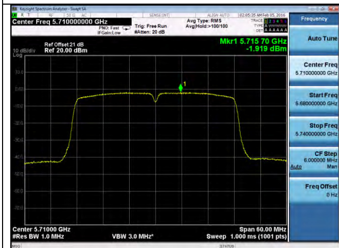
PSD-802.11n-40M-CROSS-5710M-chain3
