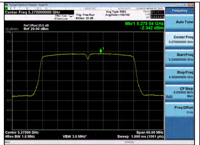
PSD-802.11n-40M-5270M-chain2
