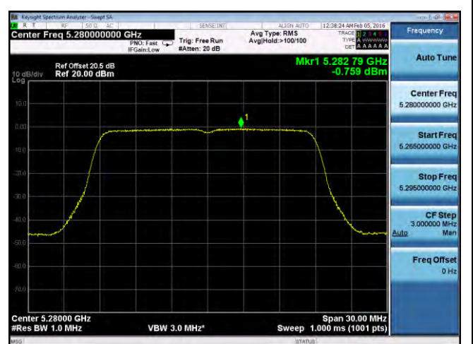
PSD-802.11n-20M-5280M-chain2
