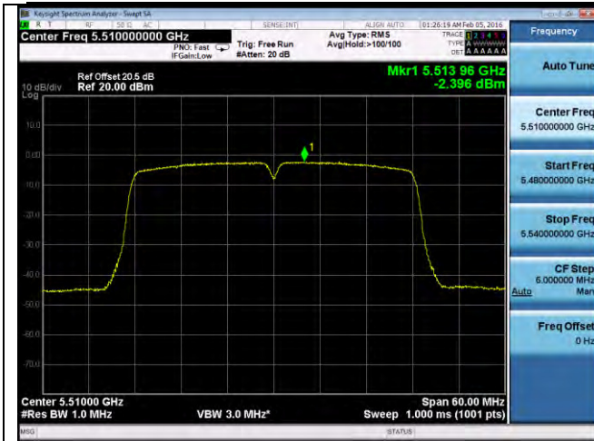
PSD-802.11n-40M-5510M-chain1
