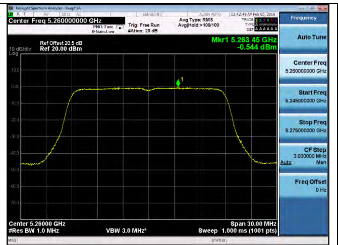
PSD-802.11n-20M-5260M-chain2
