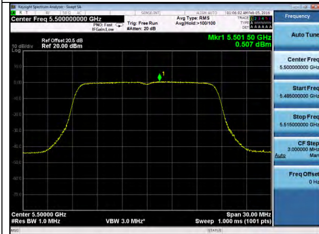
PSD-802.11a-5500M-chain3
