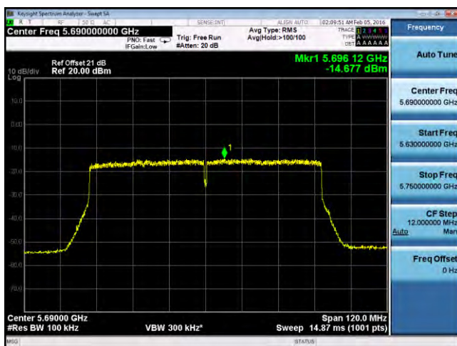
PSD-802.11ac-CROSS-5690M-chain3
