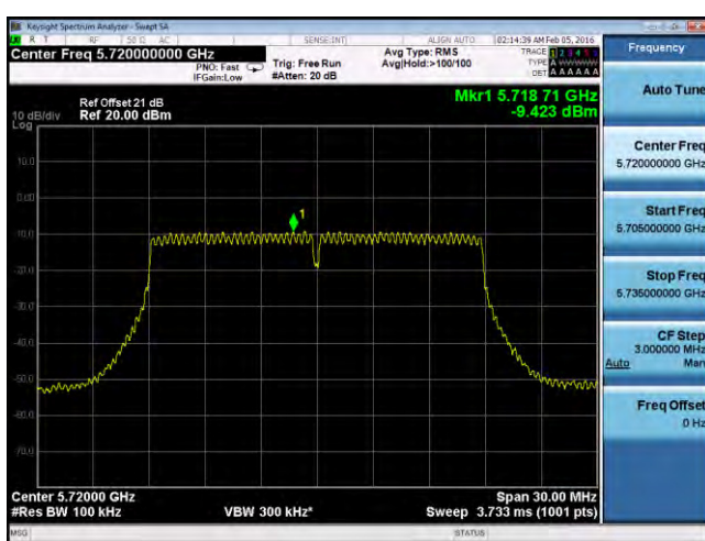
PSD-802.11n-20M-CROSS-5720M-chain3
