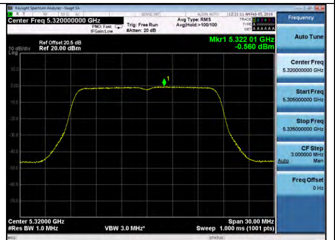
PSD-802.11a-5320M-chain2
