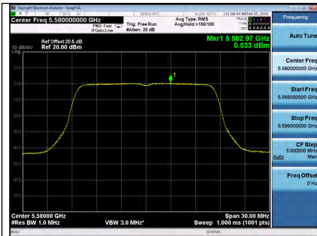
PSD-802.11a-5580M-chain3
