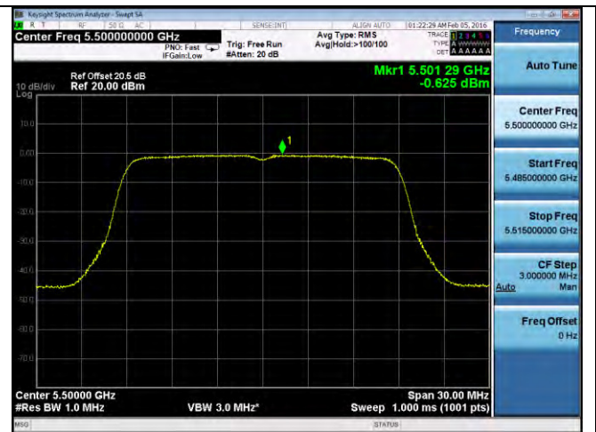
PSD-802.11n-20M-5500M-chain2
