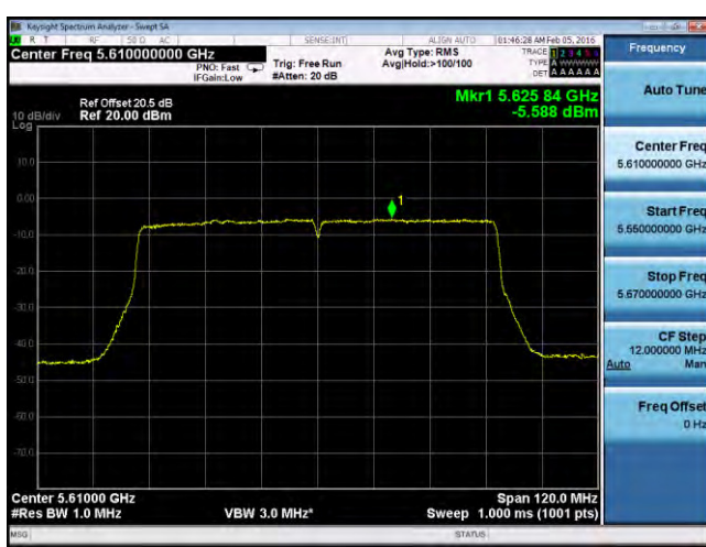
PSD-802.11ac-80M-5610M-chain3
