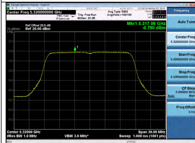
PSD-802.11a-5320M-chain1
