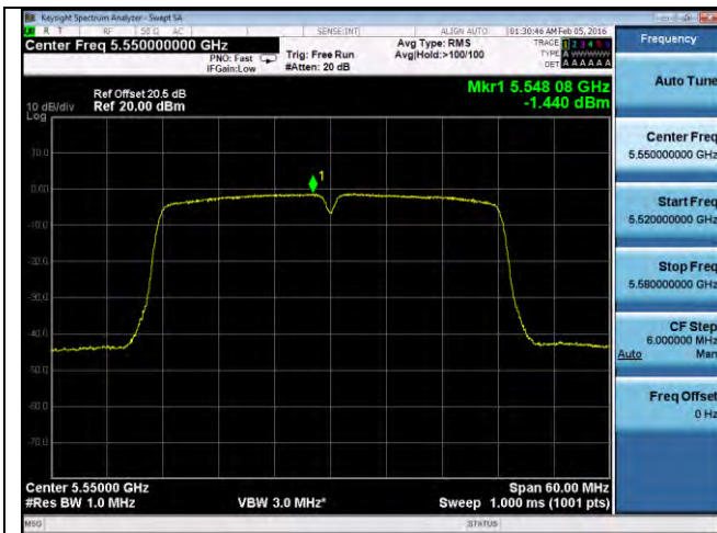
PSD-802.11n-40M-5550M-chain3
