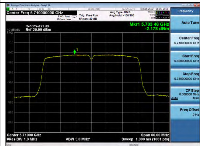
PSD-802.11n-40M-CROSS-5710M-chain4
