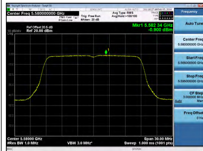
PSD-802.11n-20M-5580M-chain1
