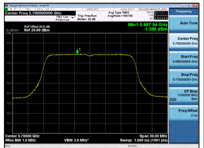
PSD-802.11a-5700M-chain4
