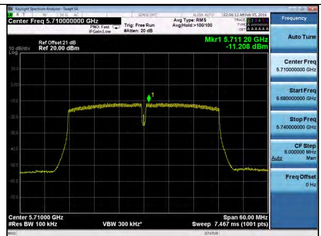
PSD-802.11n-40M-CROSS-5710M-chain4
