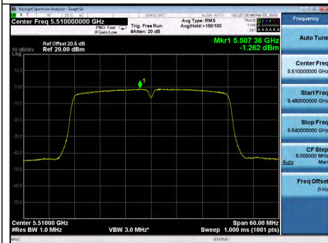
PSD-802.11n-40M-5510M-chain3
