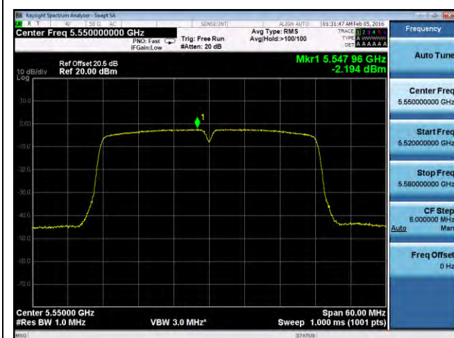
PSD-802.11n-40M-5550M-chain1
