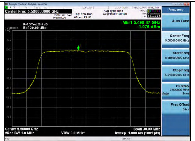
PSD-802.11n-20M-5500M-chain4
