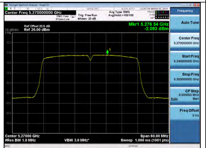
PSD-802.11n-40M-5270M-chain4
