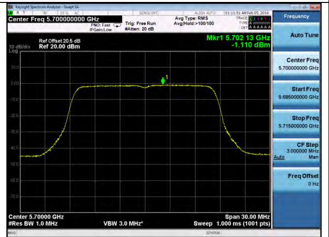
PSD-802.11a-5700M-chain2
