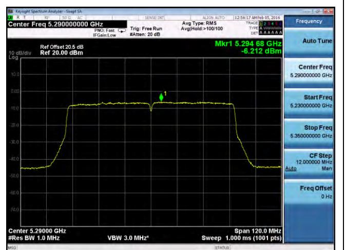
PSD-802.11ac-80M-5290M-chain4
