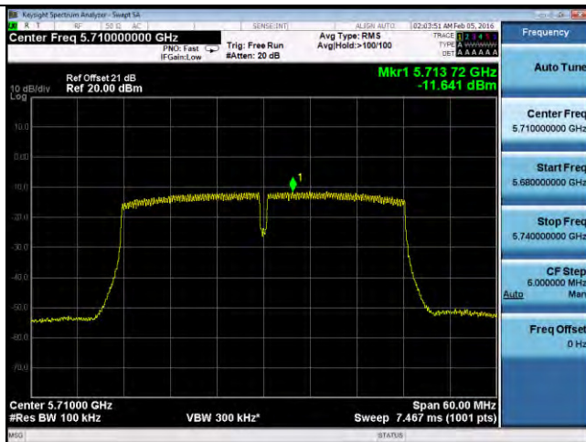
PSD-802.11n-40M-CROSS-5710M-chain1
