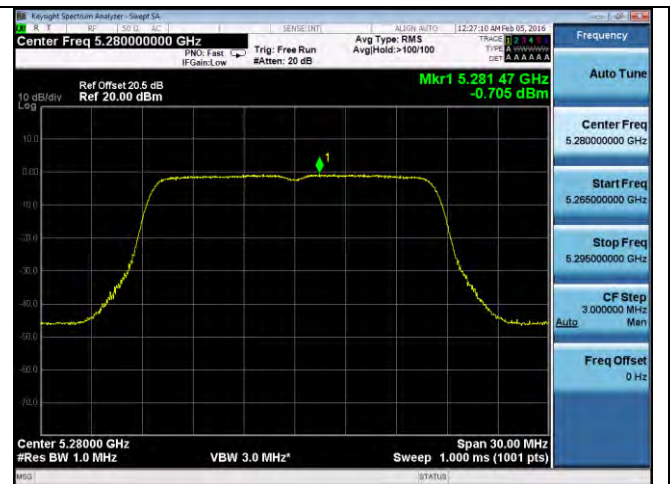
PSD-802.11a-5280M-chain4
