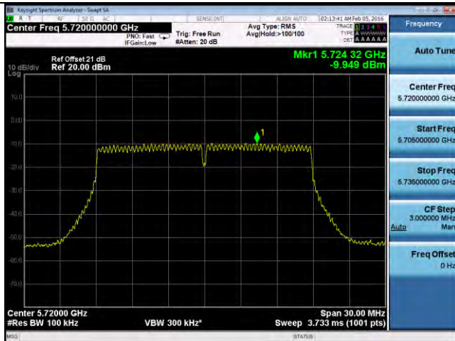
PSD-802.11n-20M-CROSS-5720M-chain1
