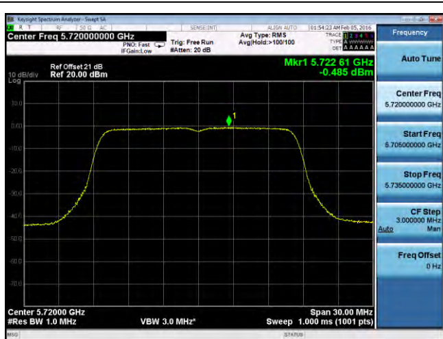
PSD-802.11a-CROSS-5720M-chain1
