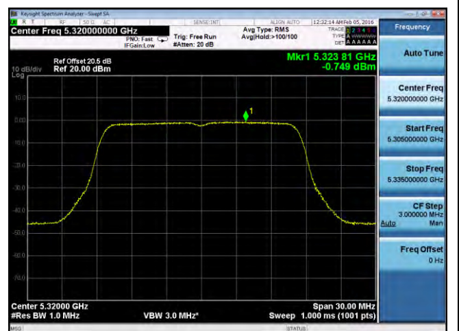
PSD-802.11a-5320M-chain4
