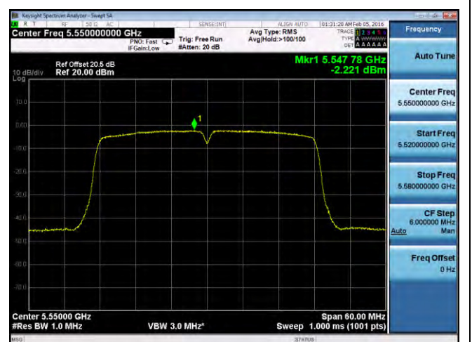
PSD-802.11n-40M-5550M-chain2
