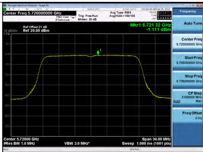
PSD-802.11n-20M-CROSS-5720M-chain1
