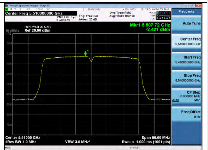
PSD-802.11n-40M-5510M-chain4
