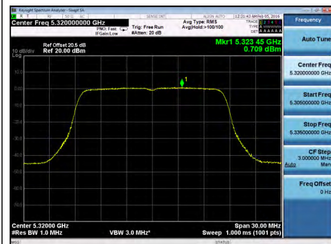
PSD-802.11a-5320M-chain3
