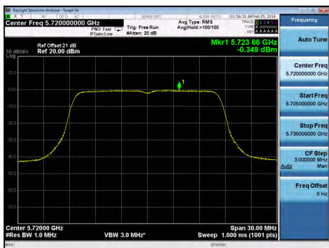
PSD-802.11a-CROSS-5720M-chain3
