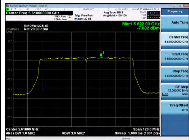
PSD-802.11ac-80M-5610M-chain1
