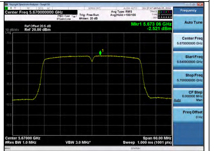
PSD-802.11n-40M-5670M-chain2
