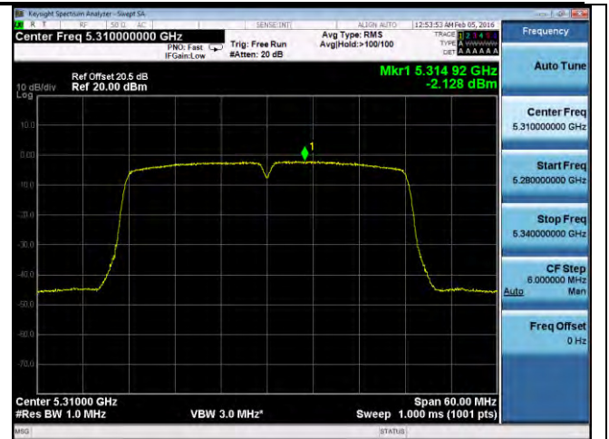
PSD-802.11n-40M-5310M-chain4
