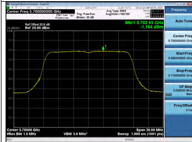
PSD-802.11a-5700M-chain1
