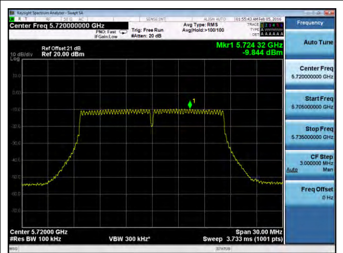
PSD-802.11a-CROSS-5720M-chain2
