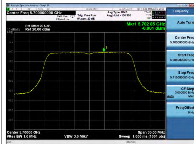
PSD-802.11a-5700M-chain3
