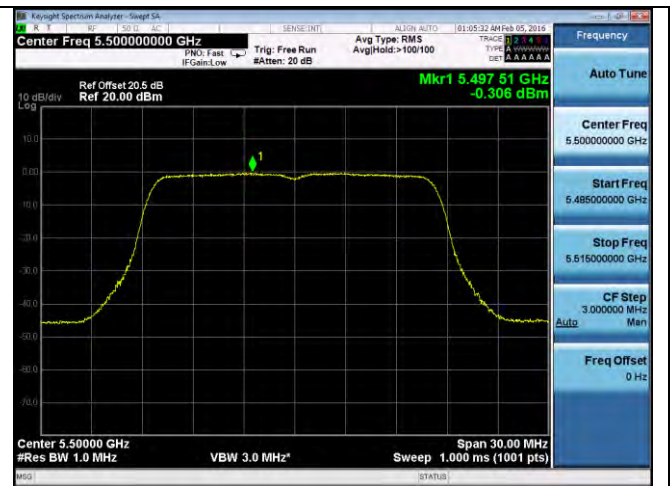
PSD-802.11a-5500M-chain2
