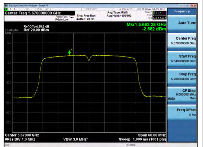
PSD-802.11n-40M-5670M-chain4
