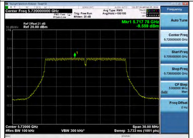
PSD-802.11a-CROSS-5720M-chain4
