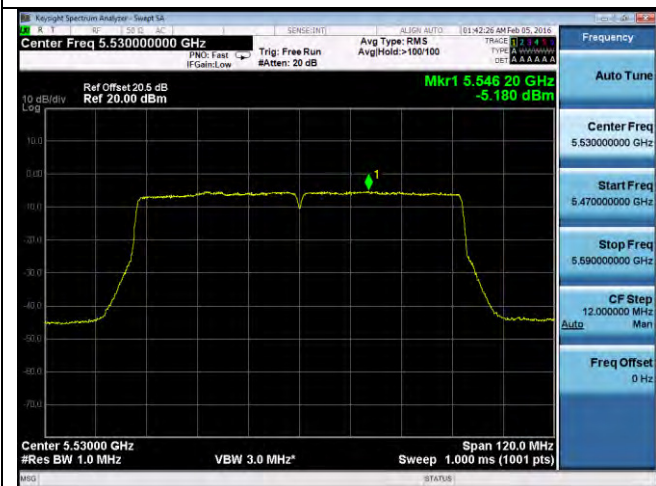
PSD-802.11ac-80M-5530M-chain3
