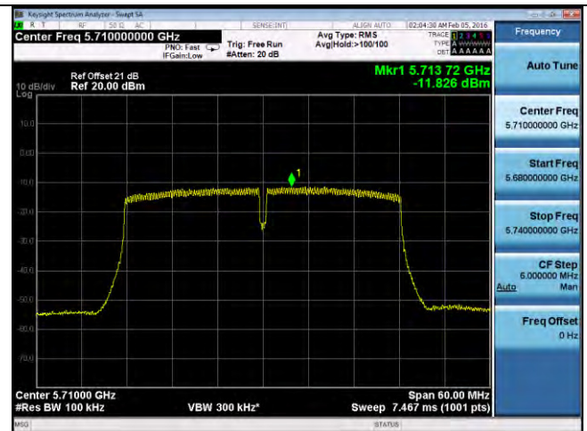
PSD-802.11n-40M-CROSS-5710M-chain2
