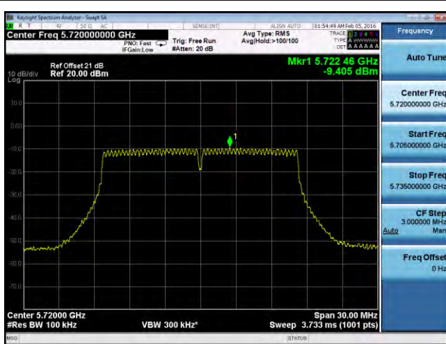
PSD-802.11a-CROSS-5720M-chain1
