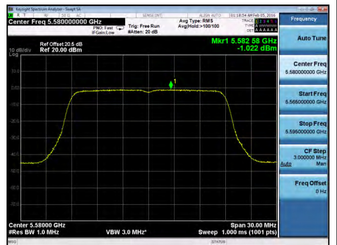
PSD-802.11n-20M-5580M-chain2
