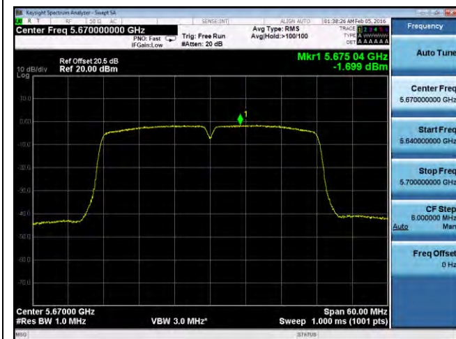
PSD-802.11n-40M-5670M-chain3
