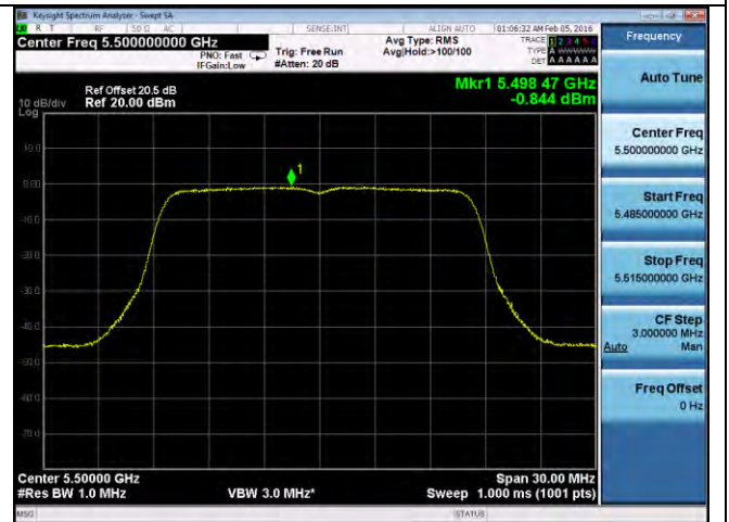
PSD-802.11a-5500M-chain4
