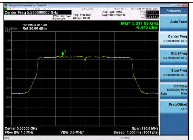
PSD-802.11ac-80M-5530M-chain4
