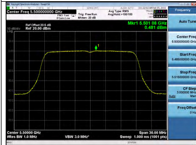
PSD-802.11n-20M-5500M-chain3
