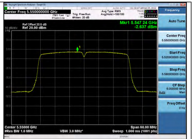
PSD-802.11n-40M-5550M-chain4
