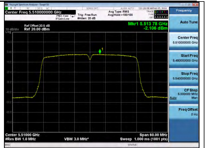
PSD-802.11n-40M-5510M-chain2
