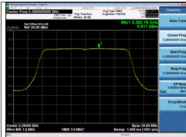
PSD-802.11n-20M-5280M-chain3
