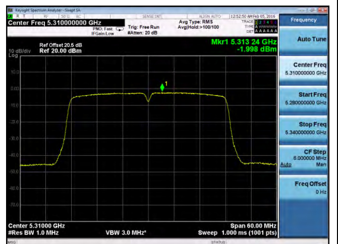
PSD-802.11n-40M-5310M-chain2
