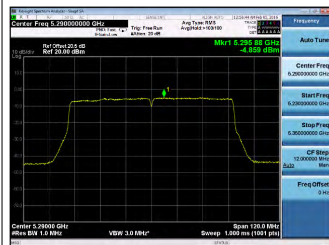
PSD-802.11ac-80M-5290M-chain3
