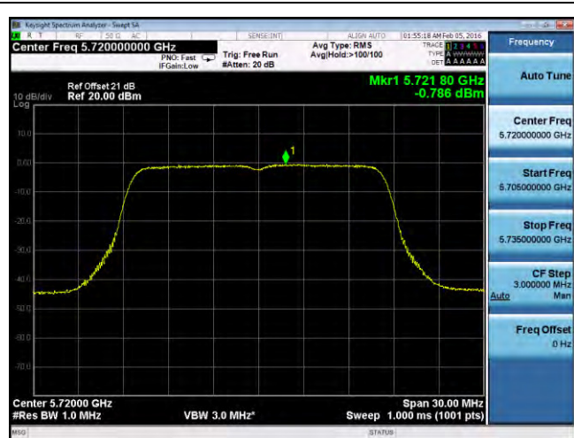
PSD-802.11a-CROSS-5720M-chain2
