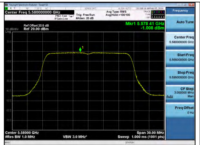
PSD-802.11a-5580M-chain4
