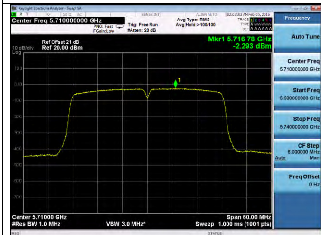
PSD-802.11n-40M-CROSS-5710M-chain1
