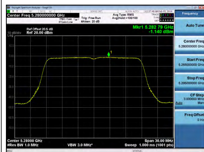
PSD-802.11n-20M-5280M-chain1
