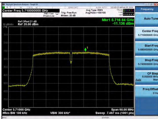
PSD-802.11n-40M-CROSS-5710M-chain3
