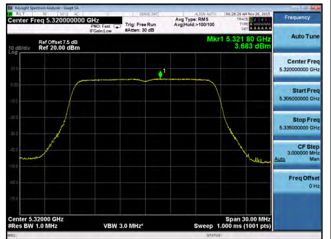
PSD-802.11a-5320M-chain4
