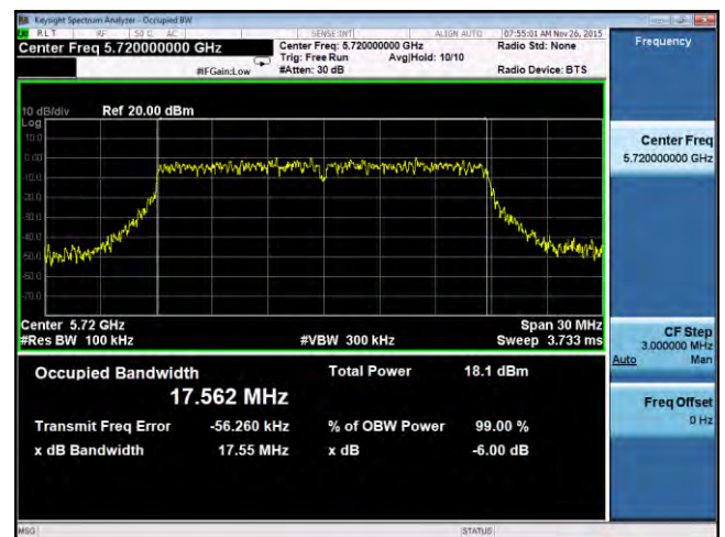
6dB BW -802.11n-20M CROSS 5720MHz
