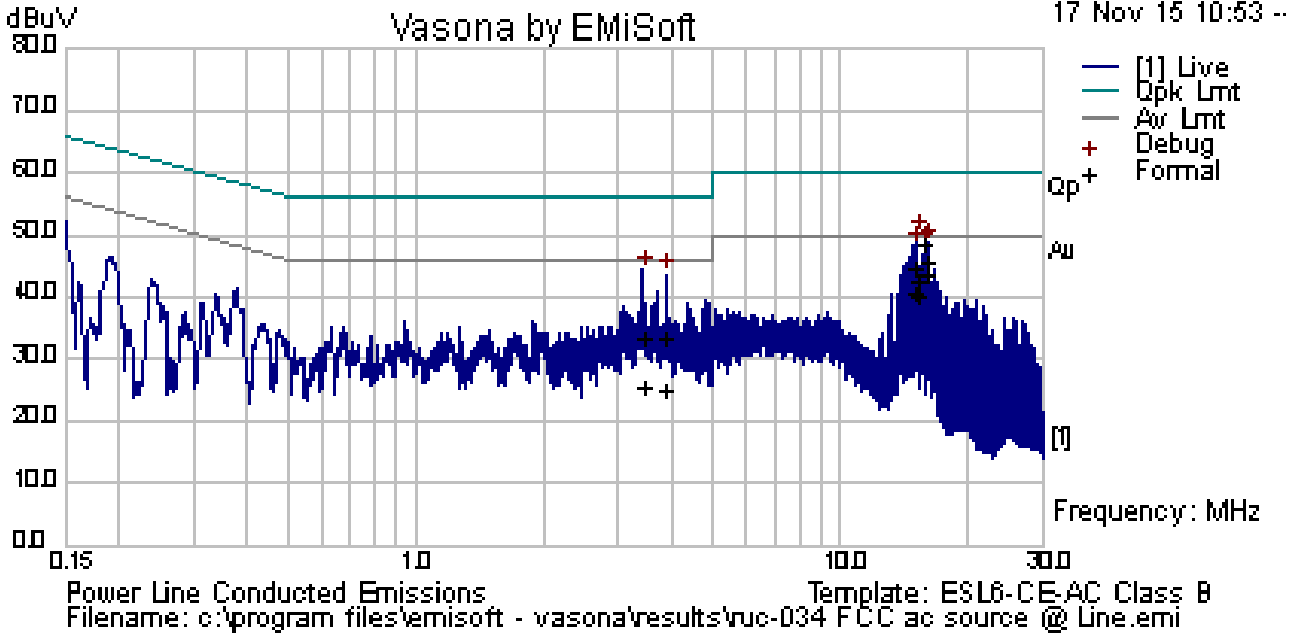
AC Line - Line Measurements @ 120V 60Hz
