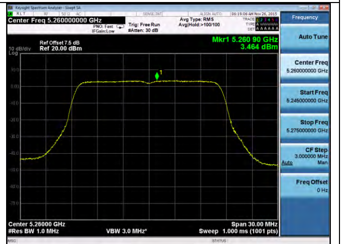
PSD-802.11a-5260M-chain4
