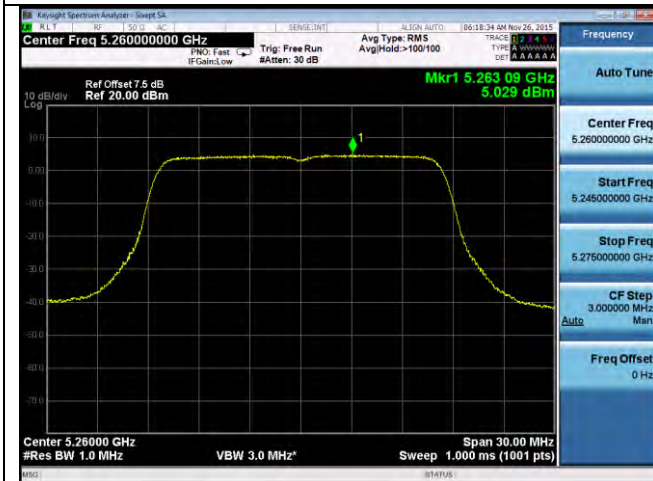
PSD-802.11a-5260M-chain3
