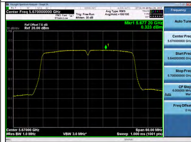
PSD-802.11n-40M-5670M-chain1
