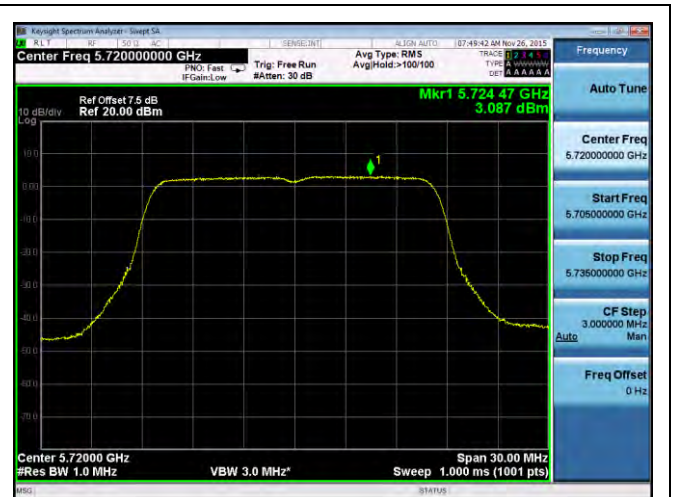
PSD-802.11a-CROSS-5720M-chain2
