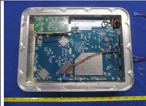
EUT Open Chassis with Antenna Board Removed
