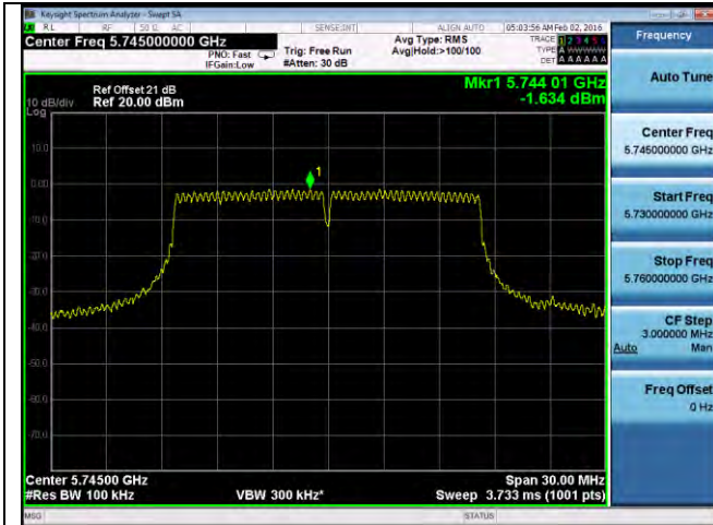
PSD-802.11a-5745M-chain1
