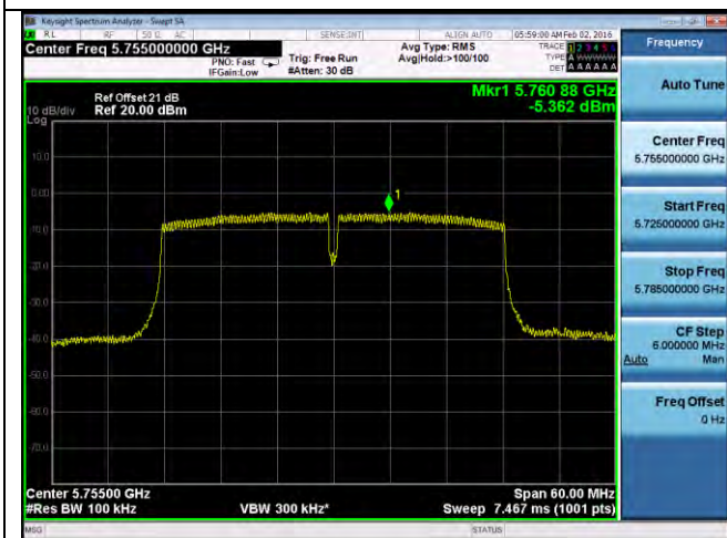
PSD-802.11n-40M-5755M-chain3
