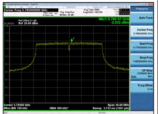
PSD-802.11a-5785M-chain2
