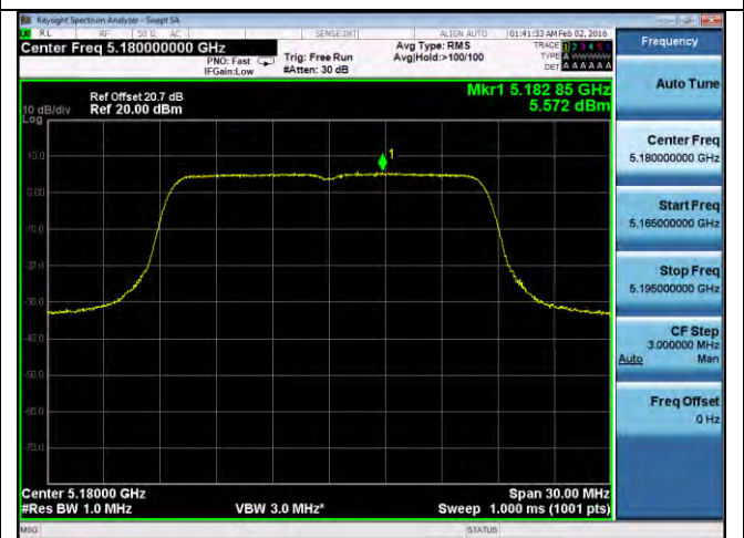
PSD-802.11a-5180M-chain4
