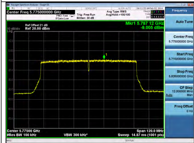
PSD-802.11ac-80M-5775M-chain3
