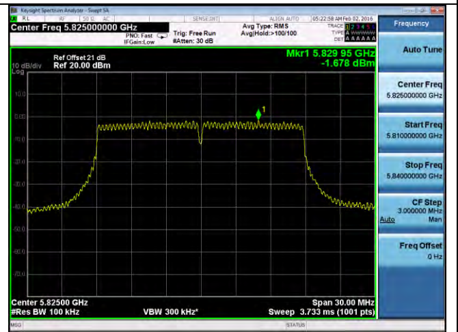
PSD-802.11n-20M-5825M-chain2
