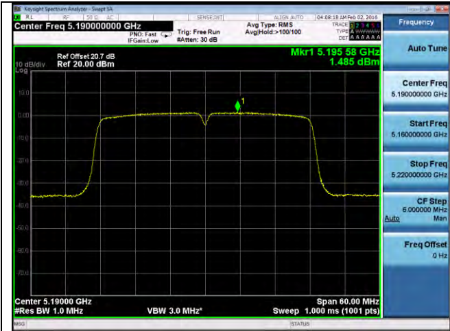
PSD-802.11n-40M-5190M-chain1
