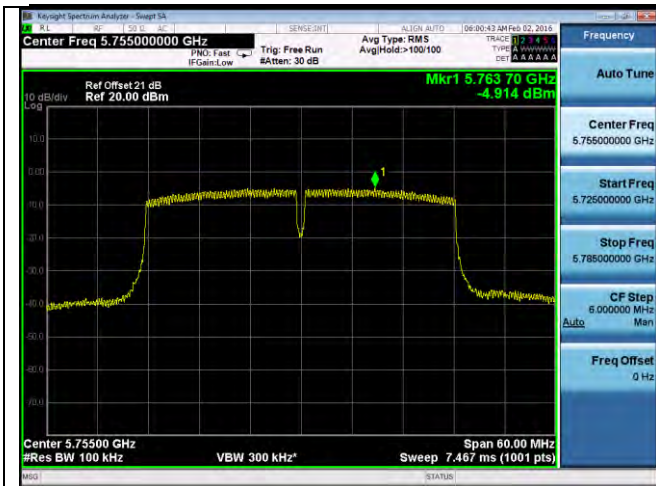
PSD-802.11n-40M-5755M-chain1
