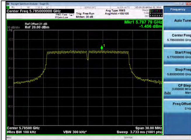
PSD-802.11a-5785M-chain3
