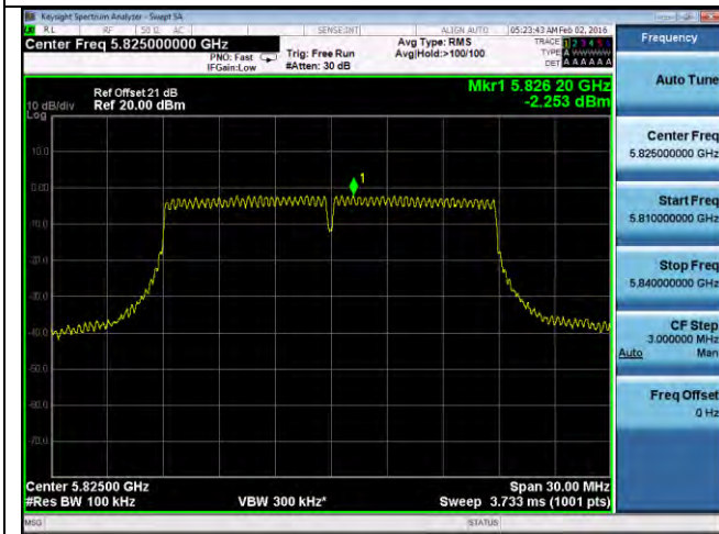
PSD-802.11n-20M-5825M-chain1
