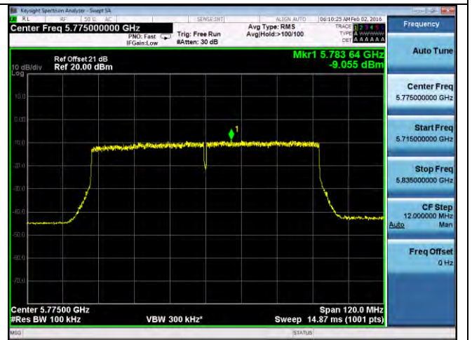
PSD-802.11ac-80M-5775M-chain2
