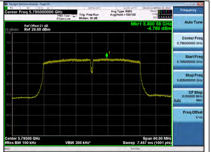
PSD-802.11n-40M-5795M-chain4
