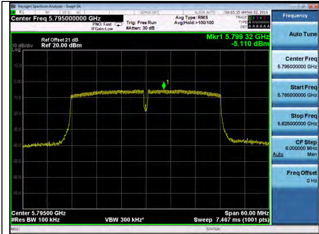
PSD-802.11n-40M-5795M-chain3
