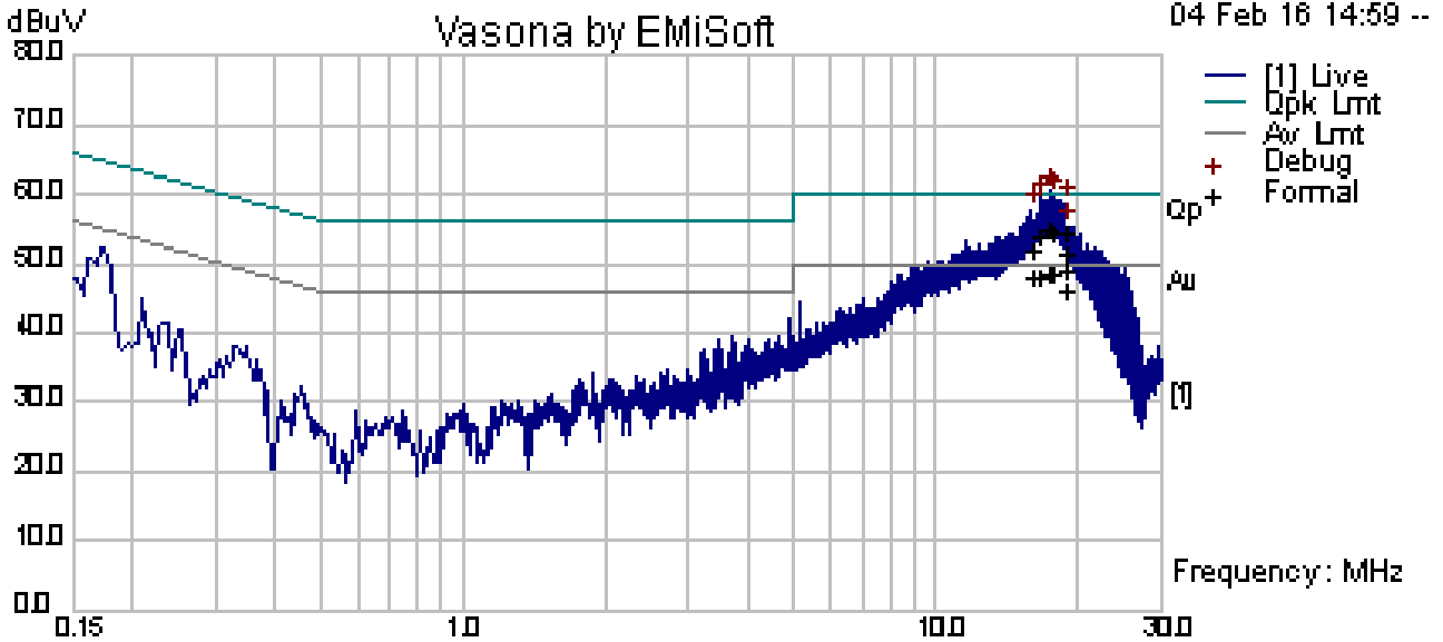
Power Line Conducted Emissions Filename: c:\program files\emisoft - vasona\results\vuc-035 source ac @live.emi Template: AC Cond Emis- Class B
