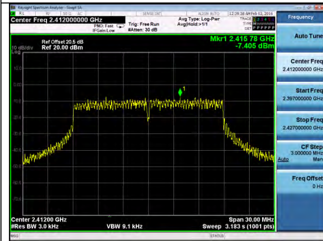
PSD-2.4G-802.11n-20M Low-chain3
