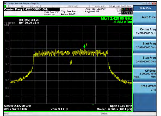
PSD-2.4G-802.11n-40M Low-chain4
