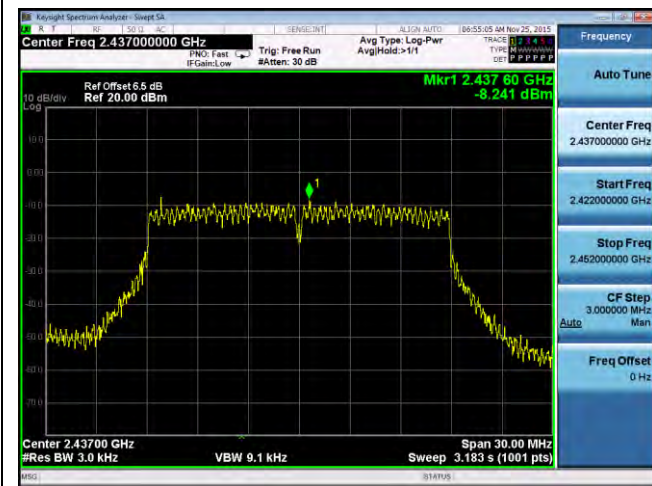
PSD-2.4G-802.11n-20M Mid-chain1
