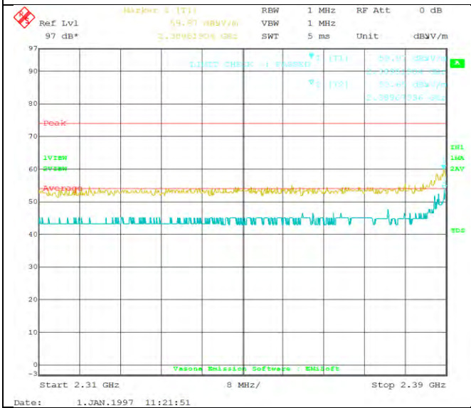
802.11n40 2422M-Restricted Band 2310-2390MHz
