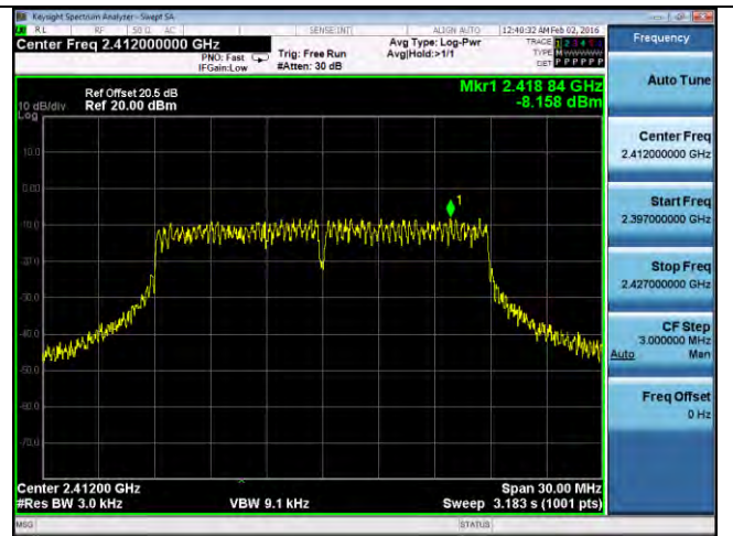
PSD-2.4G-802.11n-20M Low-chain4
