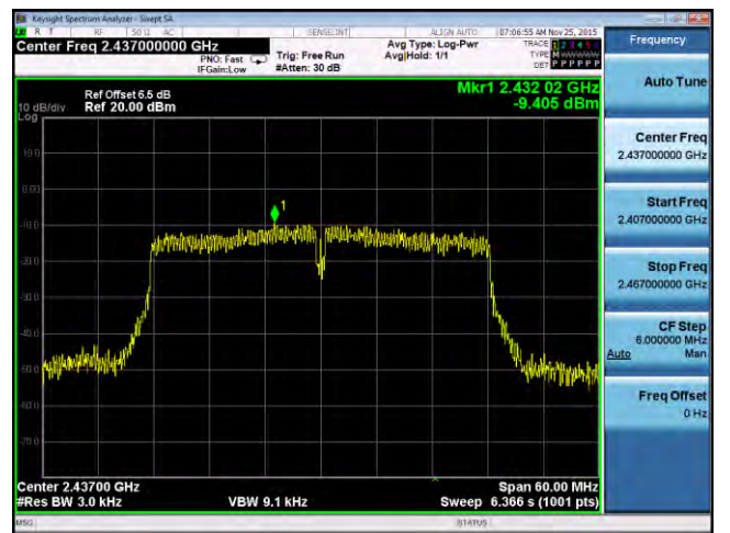
PSD-2.4G-802.11n-20M Mid-chain2
