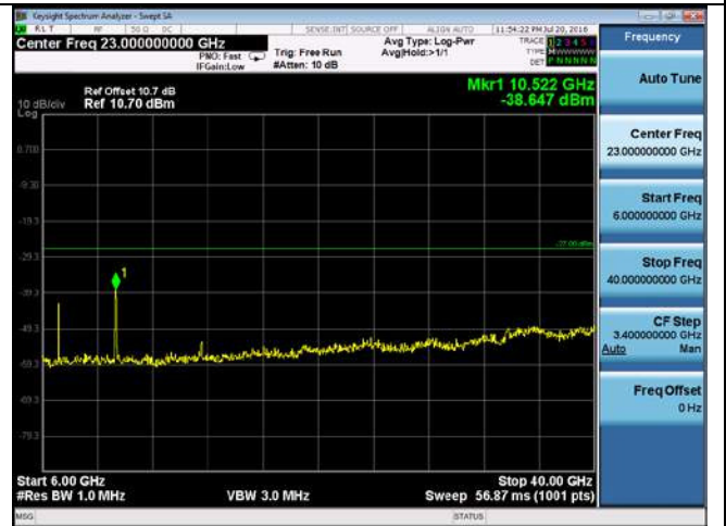
CUE-802.11n-40-5270M-chain1(6GHz-40GHz)
