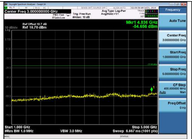
CUE-802.11n-40-5270M-chain4(1GHz-5GHz)
