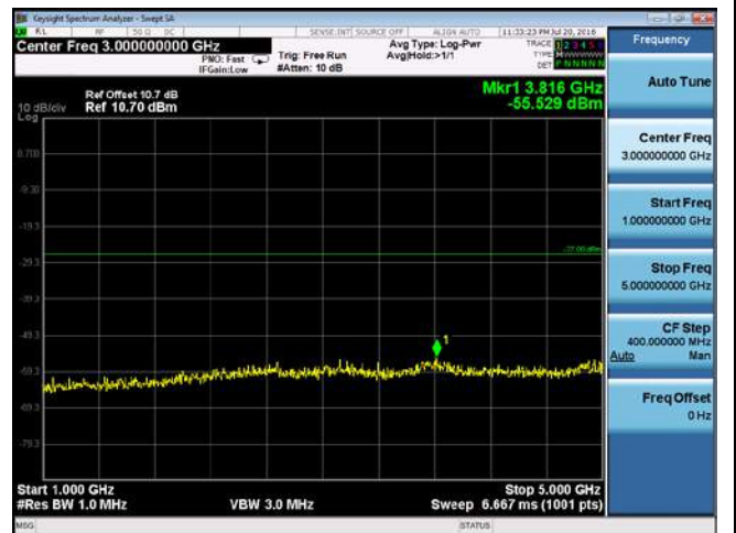
CUE-802.11n-20-5580M-chain1(1GHz-5GHz)
