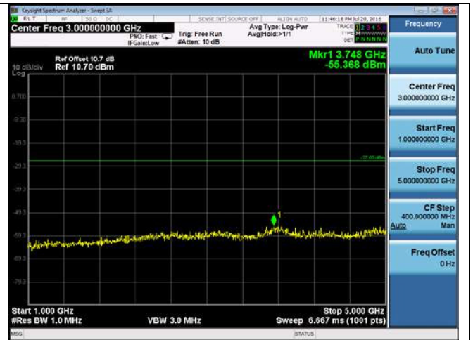
CUE-802.11n-20-5500M-chain1(1GHz-5GHz)
