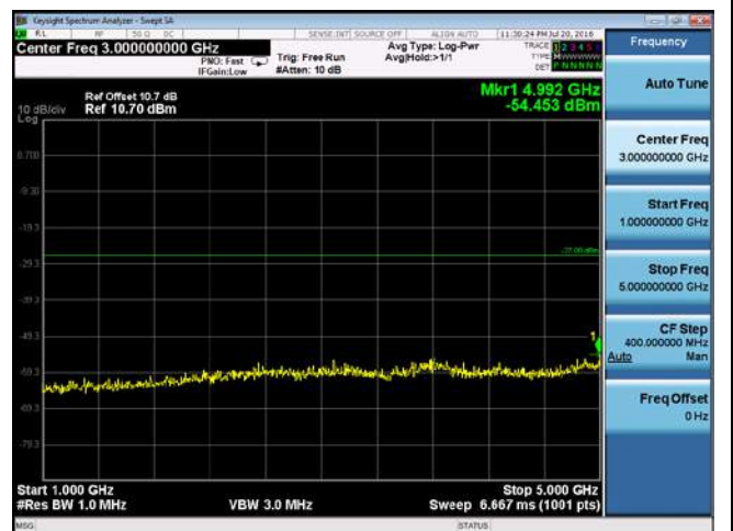
CUE-802.11a-5280M-chain1(1GHz-5GHz)
