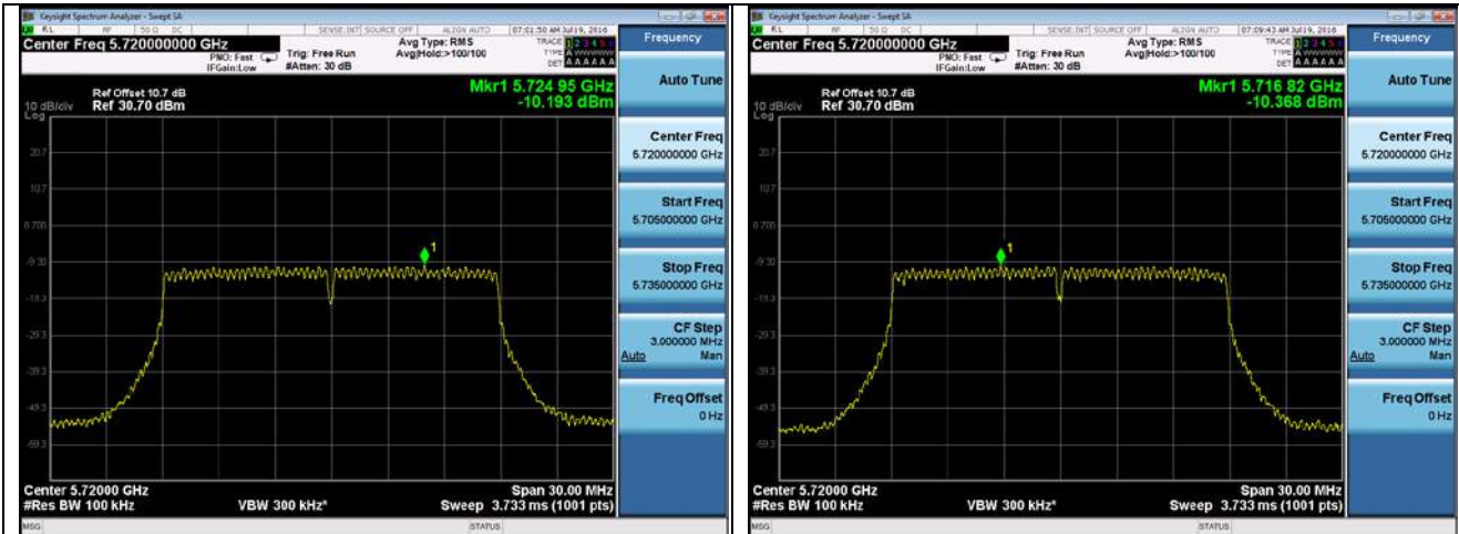
PSD-802.11n-20M-CROSS-5720M-chain3
