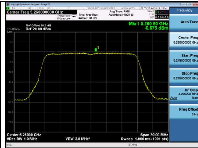
PSD-802.11n-20M-5260M-chain1
