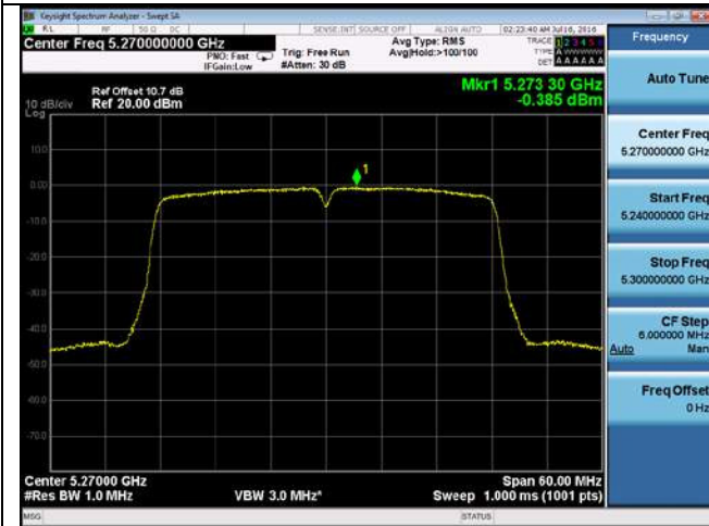
PSD-802.11n-40M-5270M-chain3
