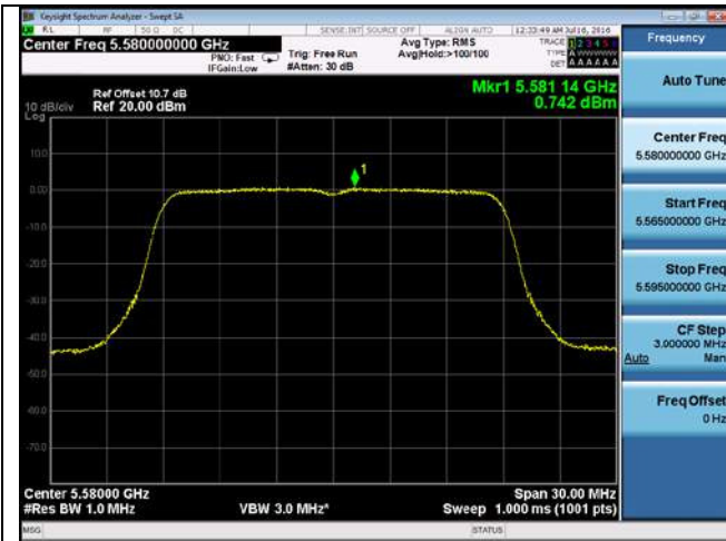
PSD-802.11n-20M-5580M-chain3
