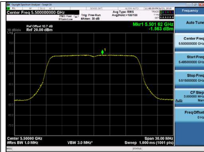
PSD-802.11a-5500M-chain1
