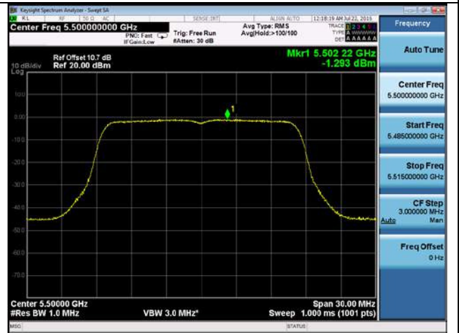
PSD-802.11a-5500M-chain4
