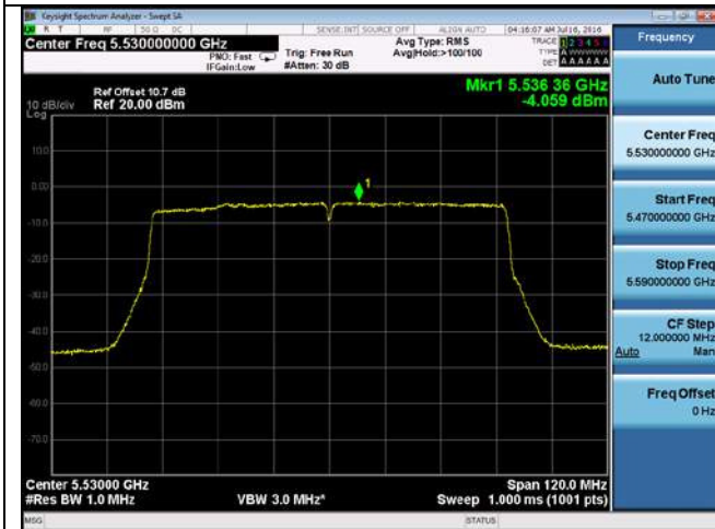
PSD-802.11ac-80M-5530M-chain3
