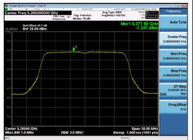
PSD-802.11a-5280M-chain2
