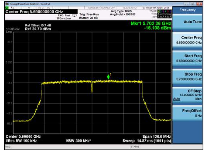
PSD-802.11ac-CROSS-5690M-chain4
