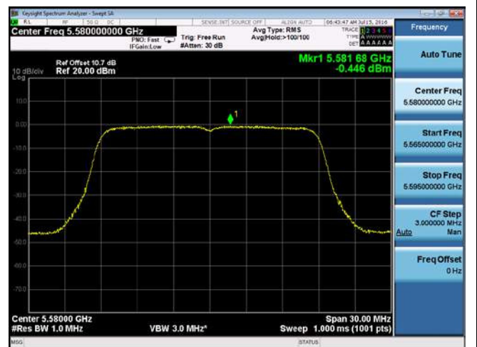
PSD-802.11n-20M-5580M-chain2
