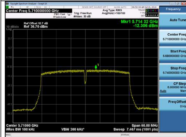
PSD-802.11n-40M-CROSS-5710M-chain1
