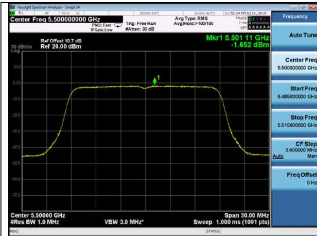
PSD-802.11n-20M-5500M-chain1
