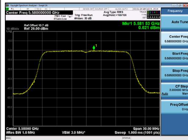
PSD-802.11n-20M-5580M-chain1
