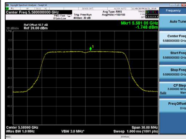
PSD-802.11a-5580M-chain1
