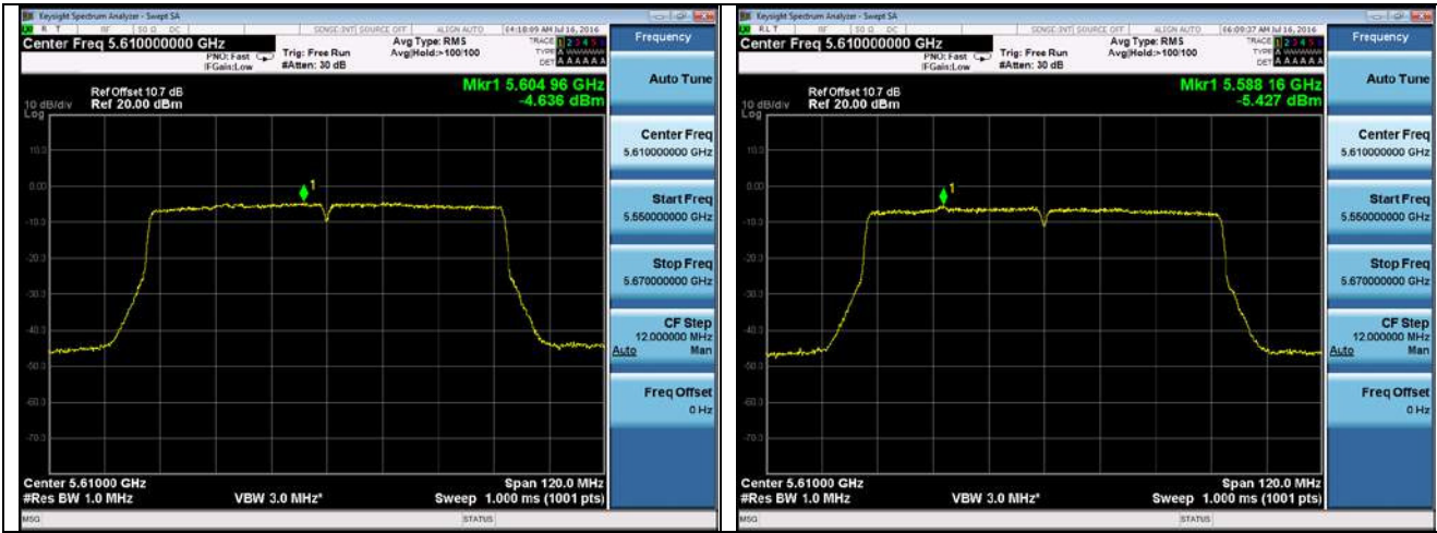
PSD-802.11ac-80M-5610M-chain3
