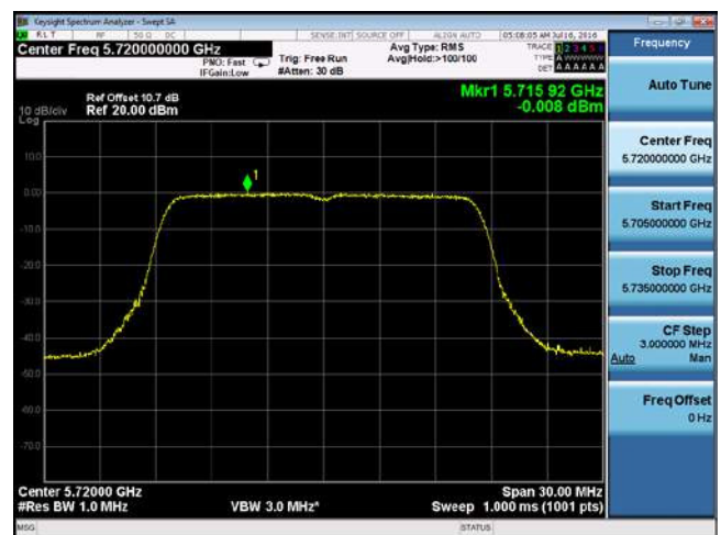
PSD-802.11a-CROSS-5720M-chain4
