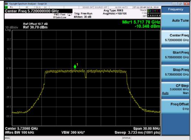
PSD-802.11a-CROSS-5720M-chain4
