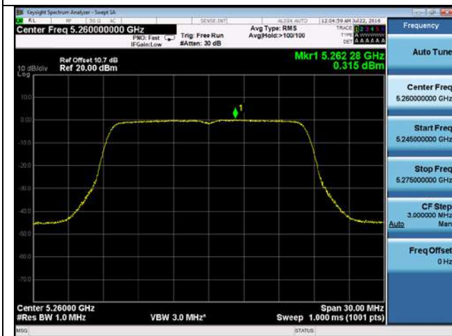
PSD-802.11a-5260M-chain3
