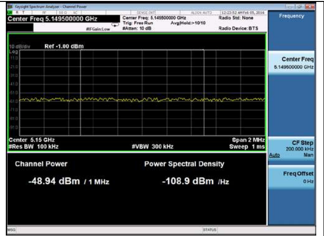
Band Edge-802.11a-5260M-chain2
